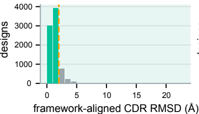
TcdB (6923/8000 < 2)
