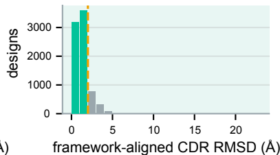
SARS-CoV-2 RBD (7246/8000 < 2)
