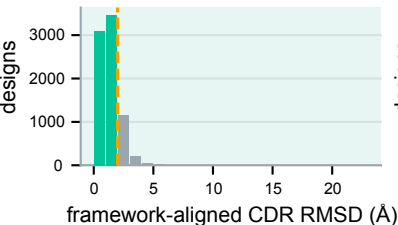
TcdB (6923/8000 < 2)
