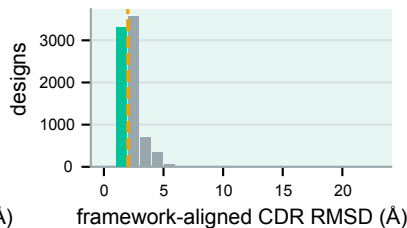
TcdB scFv unique (3319/8000 < 2)
