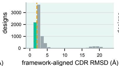
TcdB scFv comb. (2165/8000 < 2)
