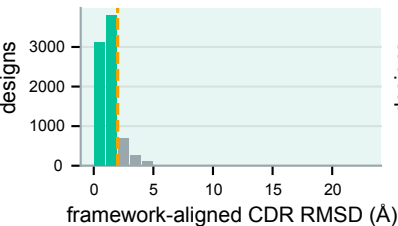
RSV-F Site I (6555/8000 < 2)
