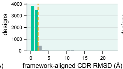
RSV-F Site III (6357/8000 < 2)
