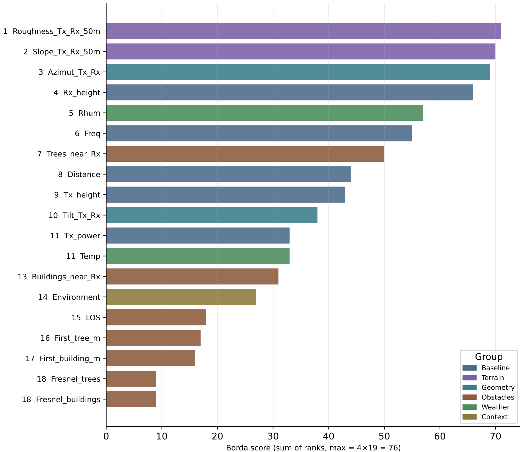
Borda consensus — out-of-fold importance in Dev
