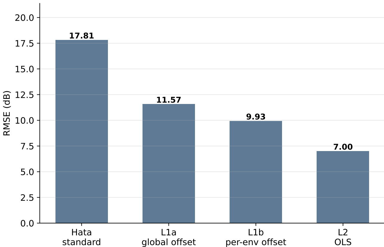
Progressive Hata calibration RMSE Test set ( d \geq 1 km, sealed)
