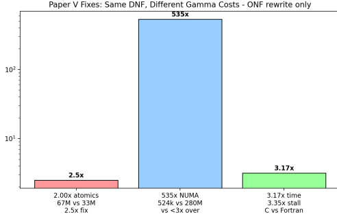
Fig. 4. Paper V results reproduced. 2.00x atomics to 2.5x via private acc, 535x NUMA vs \text{;3x} via \text{proc\_bind(close)} , 3.17x/3.35x C vs Fortran row vs col. ONF rewrite only, DNF fixed.
