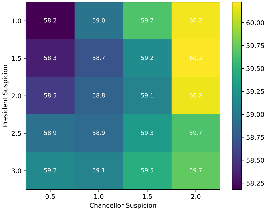
Combined Win Rate (%)
