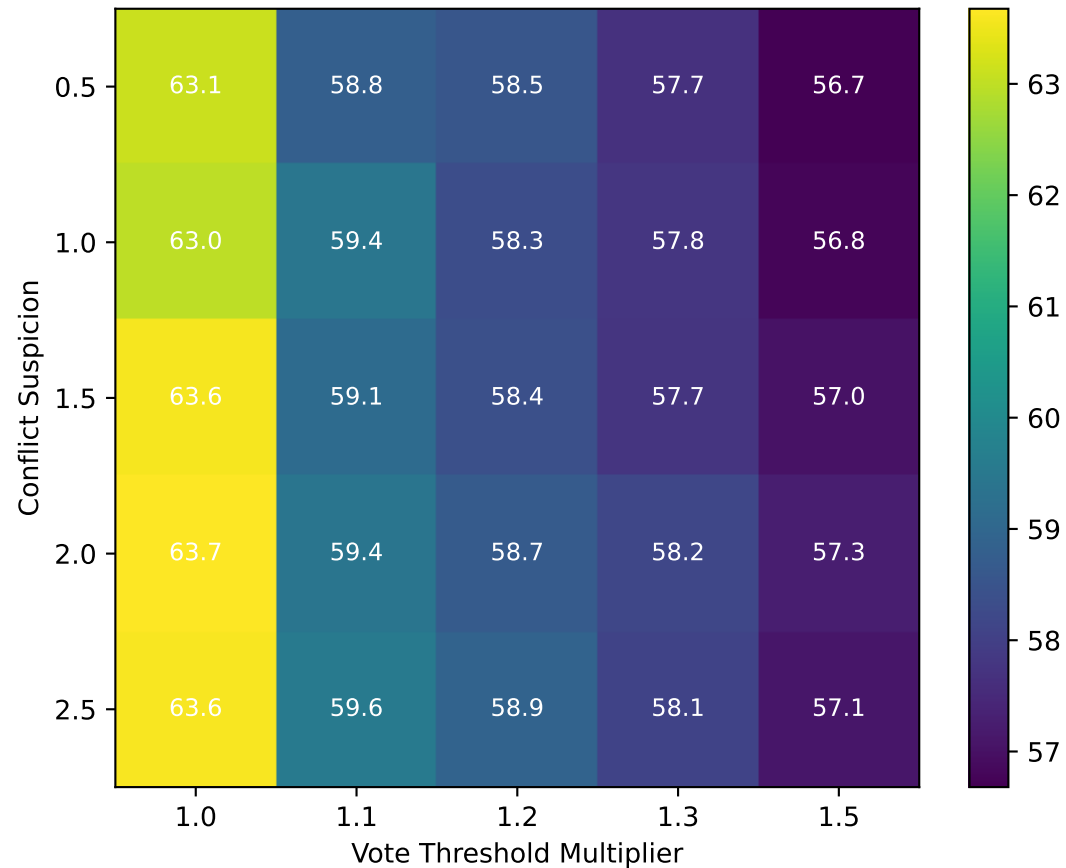
Combined Win Rate (%)
