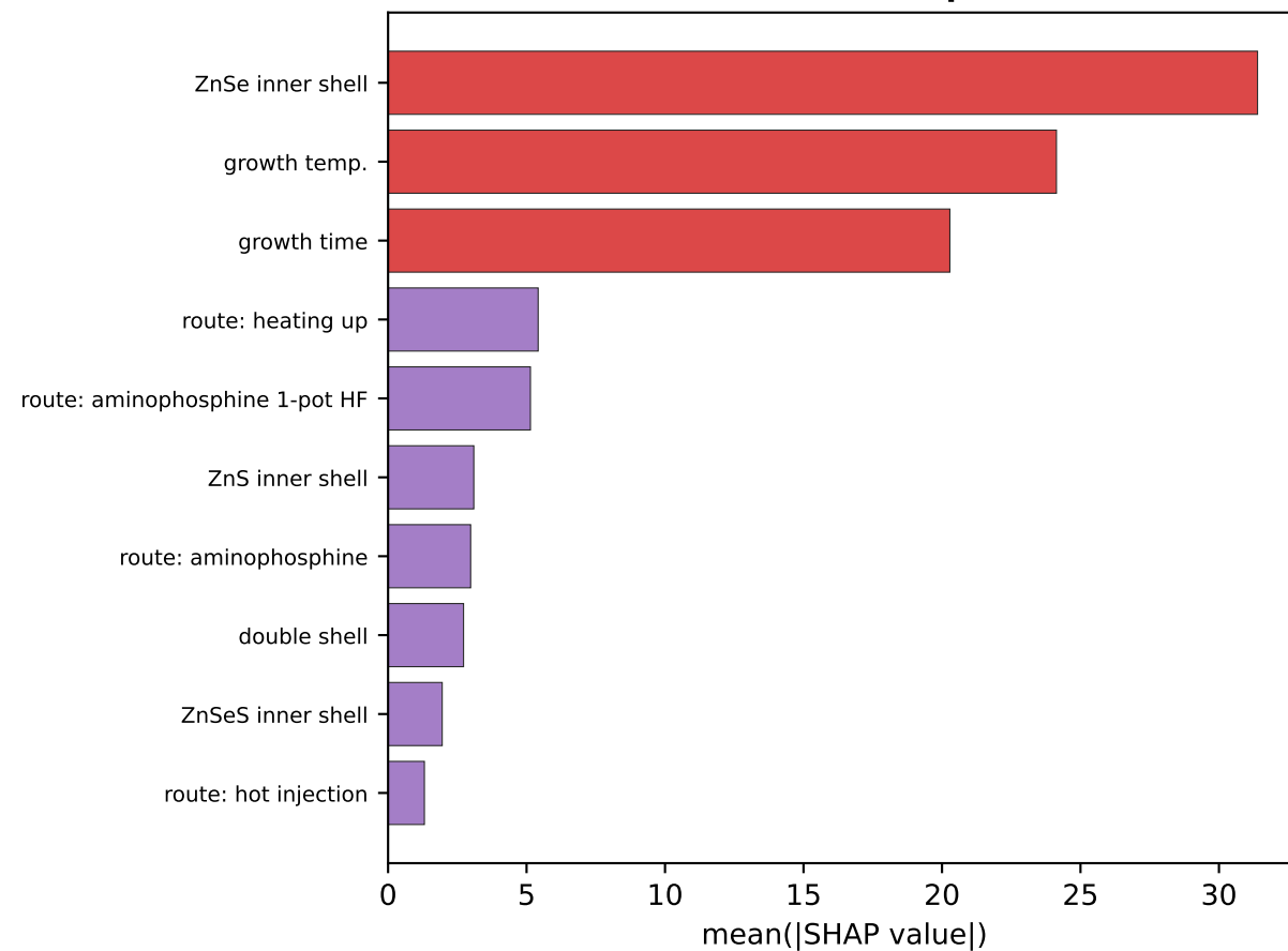
C. GBM SHAP top-10
