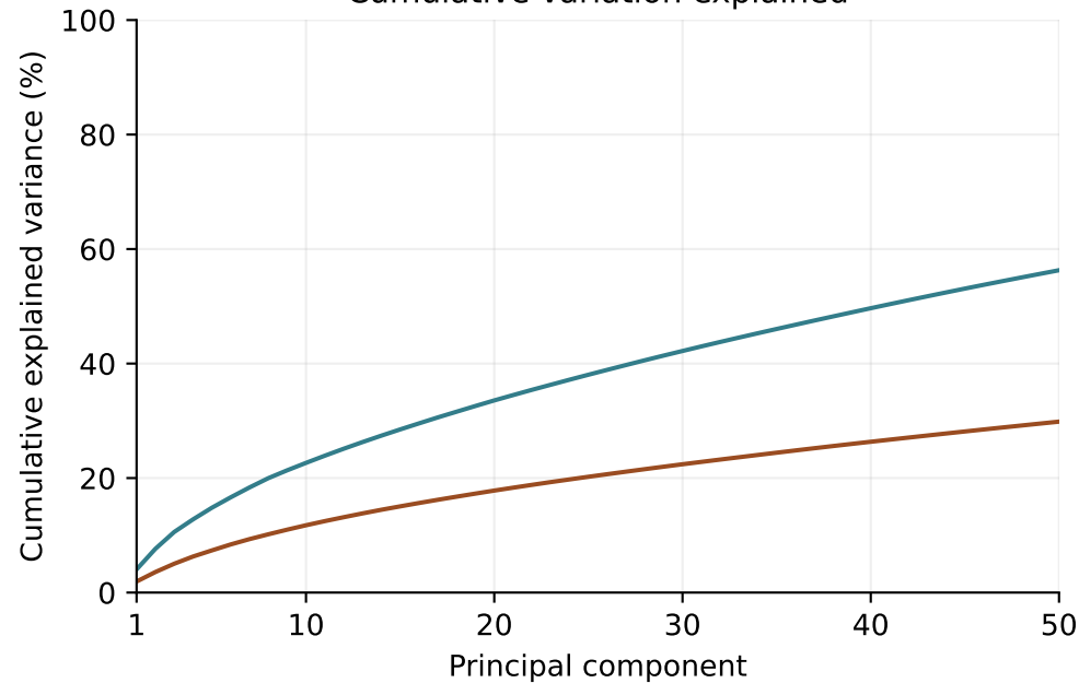
Cumulative variation explained
