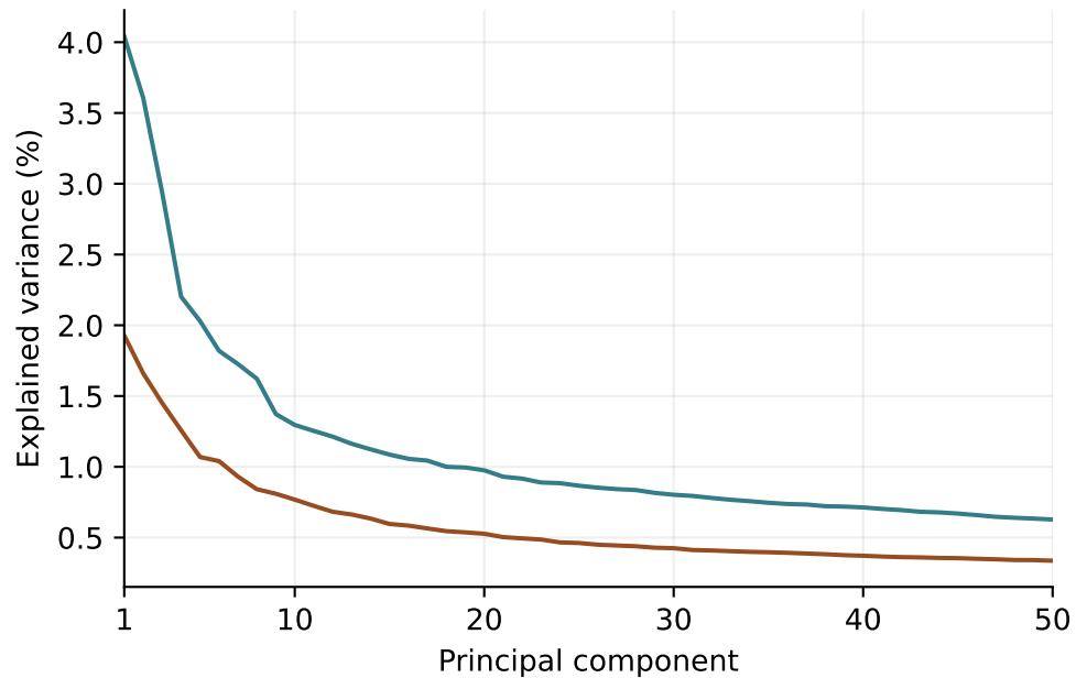
Variation explained by each component
