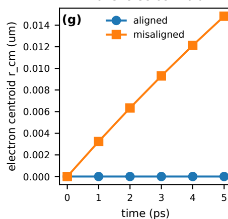
transverse centroid
