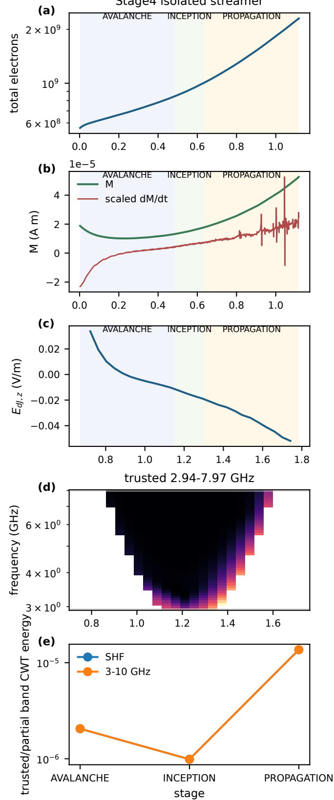
Stage4 isolated streamer
