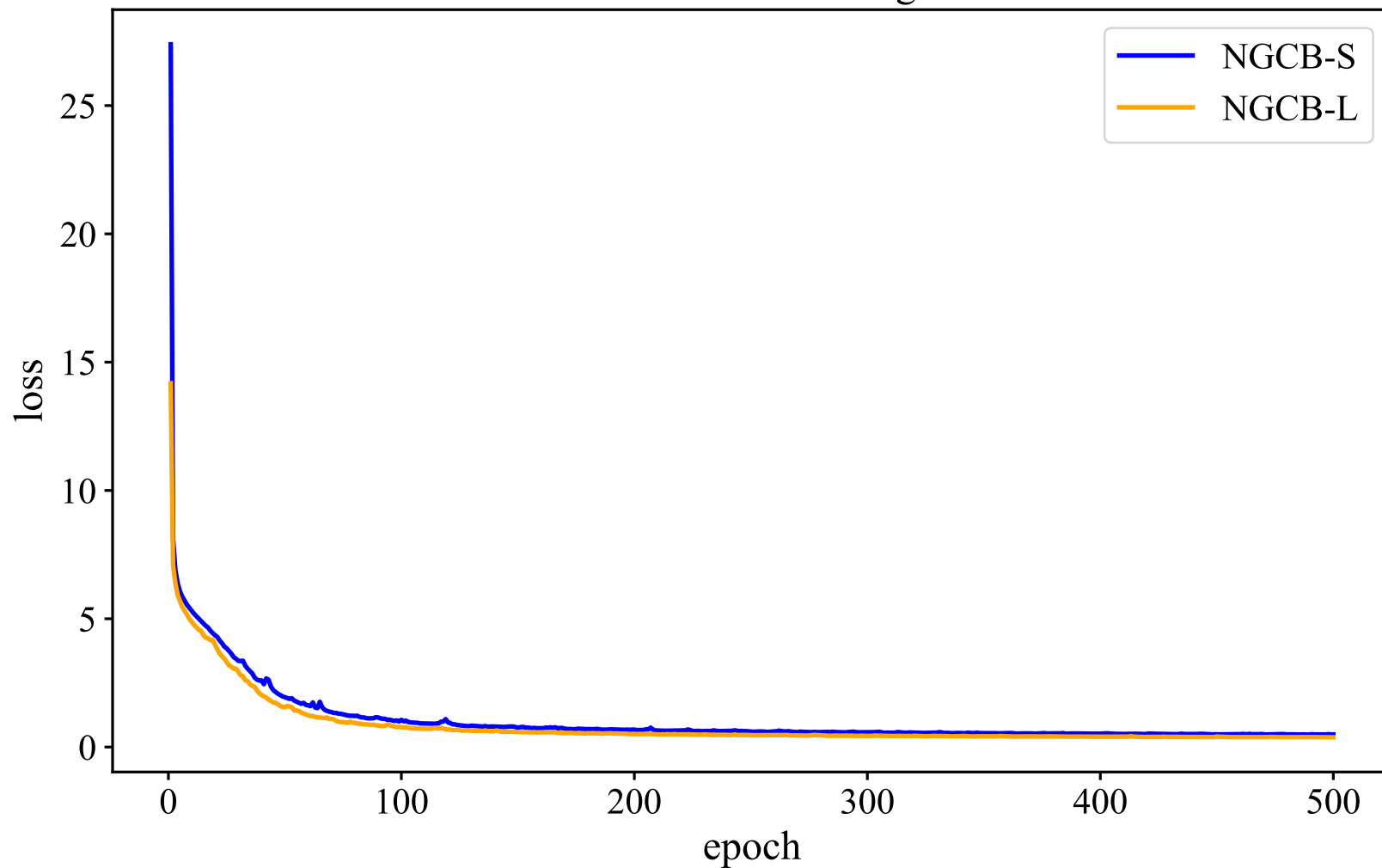
Neural Network Training Loss
