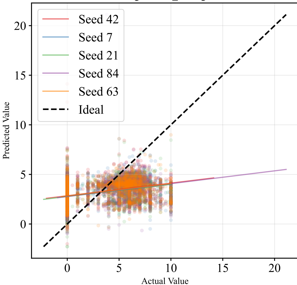
Ridge - Vote_average
