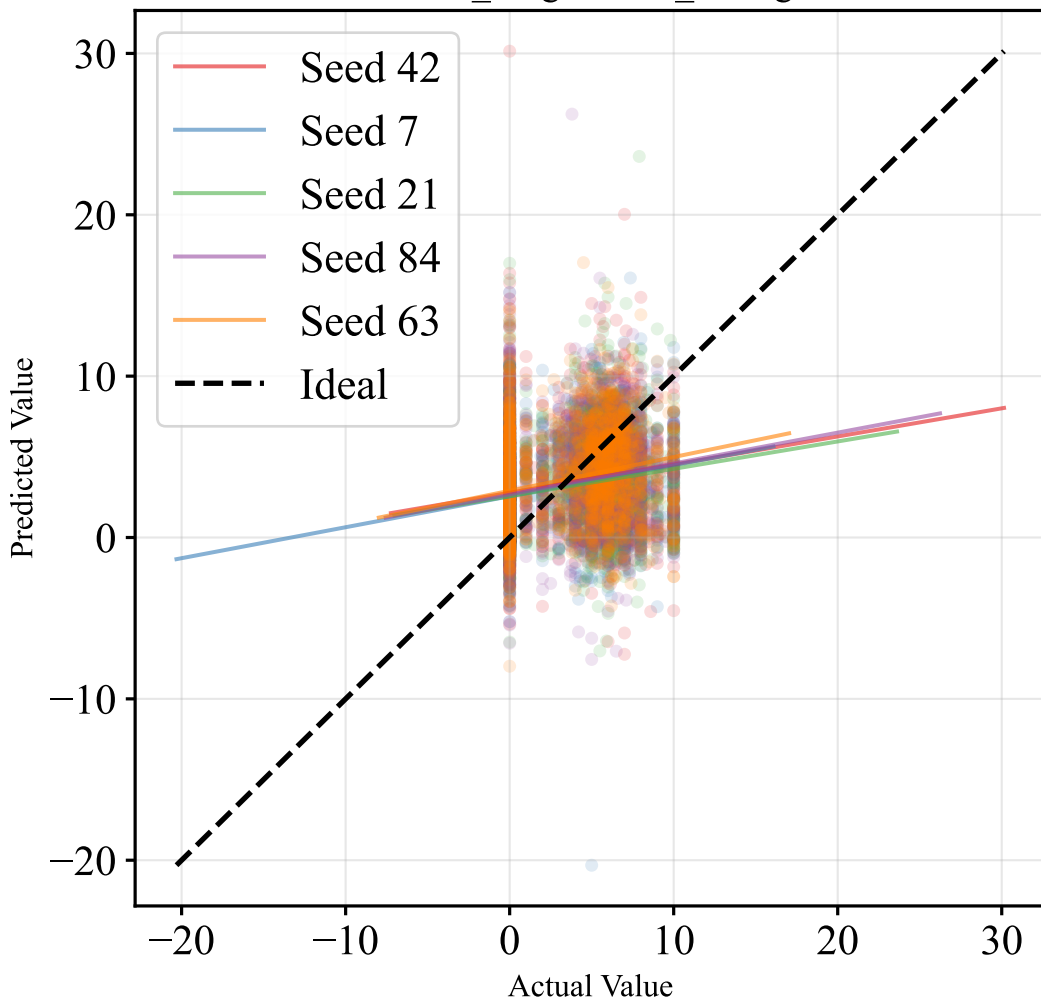
Neural_Large - Vote_average
