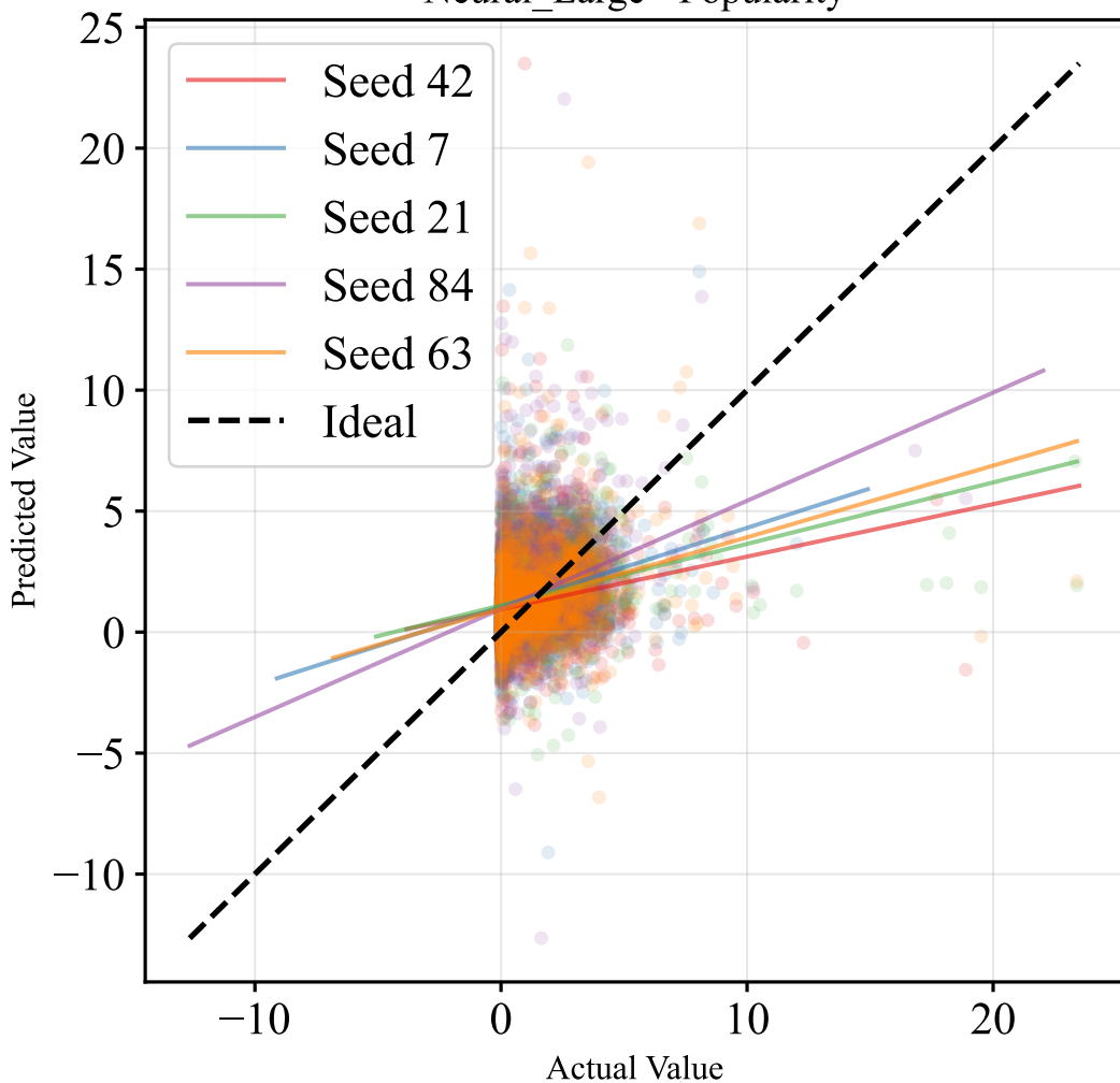
Neural_Large - Popularity
