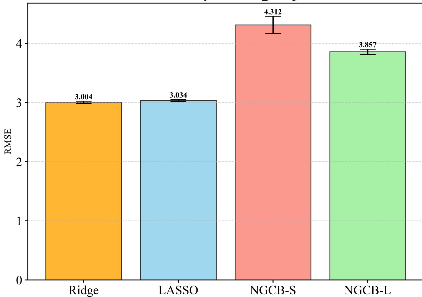
RMSE Comparison: Vote_average
