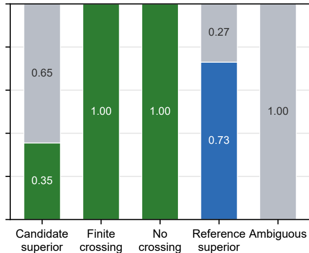
(B) Covariate-dependent censoring
