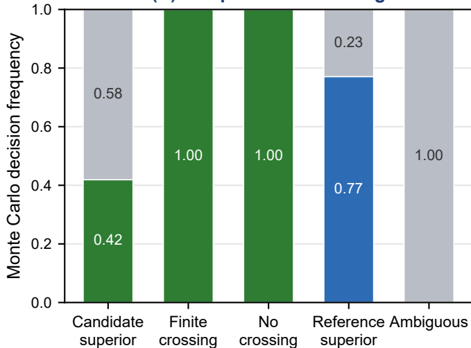
(A) Independent censoring
