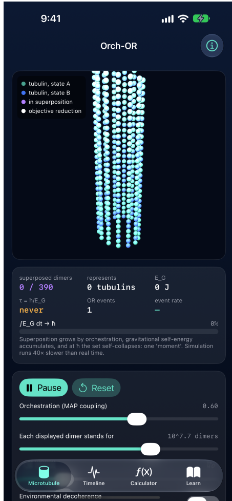
Figure 1: Left: the microtubule lattice and live readouts on iPhone. Right: coherence over simulated time with objective-reduction events (white lines) on iPad; at the default calibration the model settles near 25–28 ms per event.
