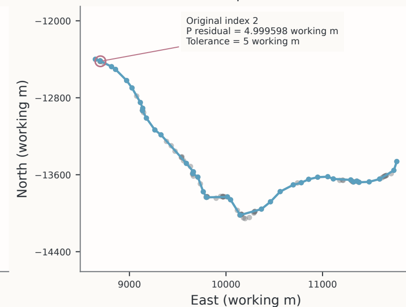
Nearest positive P residual gap record 7027 · 107 → 38 points
