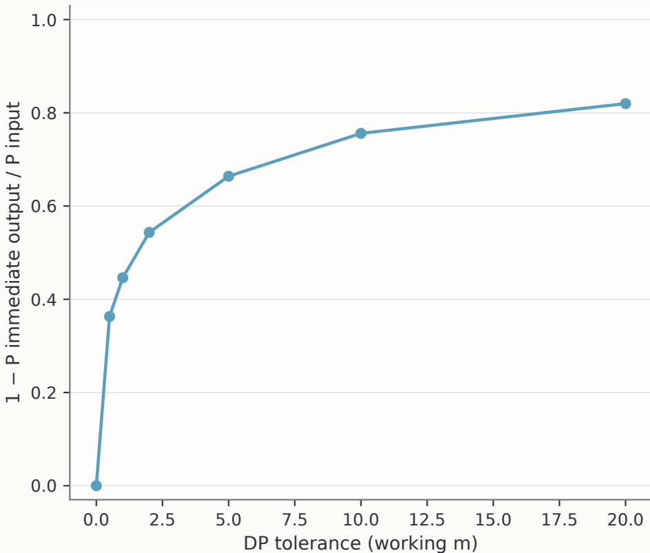
DP geometric error and compression · identical S/D input
