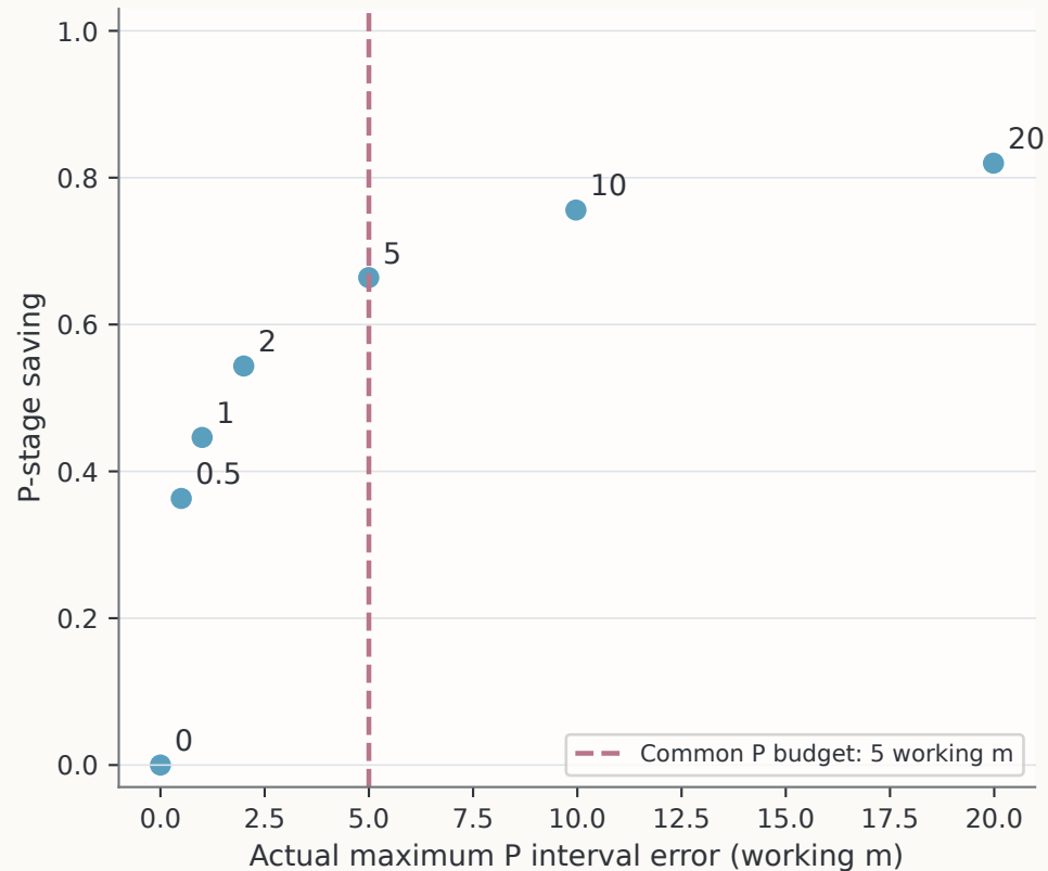
DP geometric error and compression · identical S/D input
