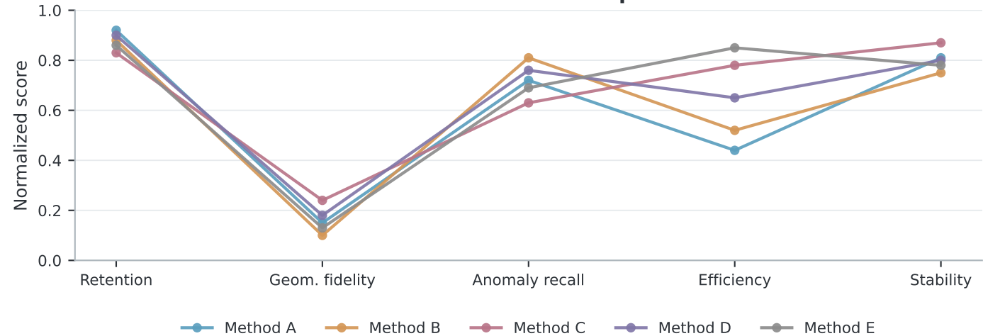
Parallel coordinates · multi-metric method comparison
