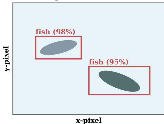
(c) In-situ Optical Data (ML Detection)
