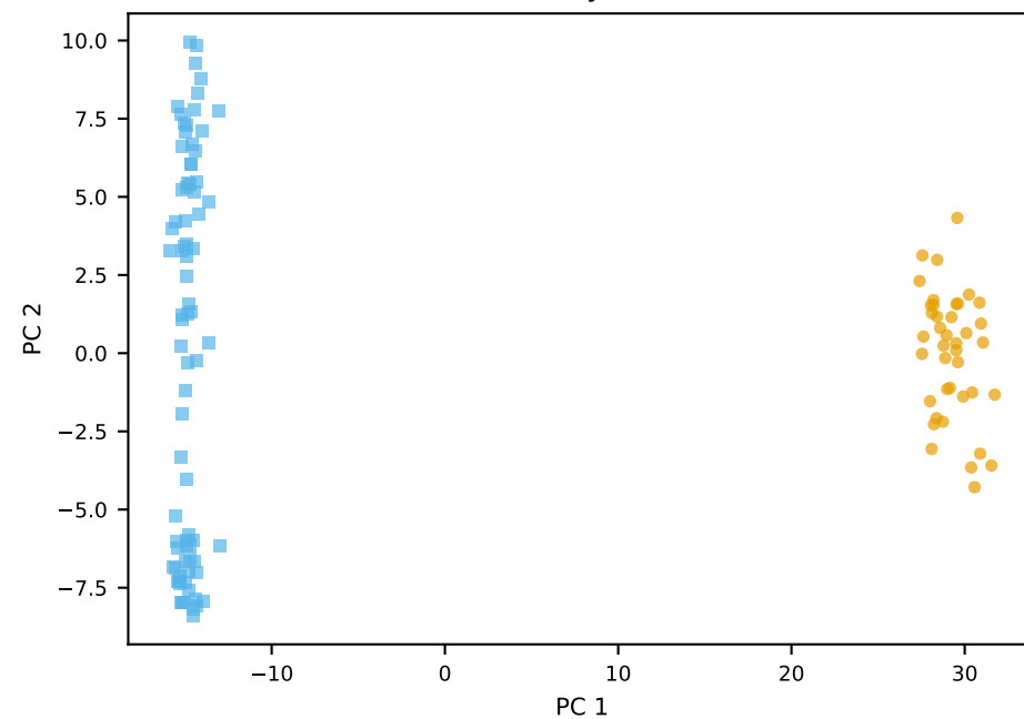
Cross-study encoder
