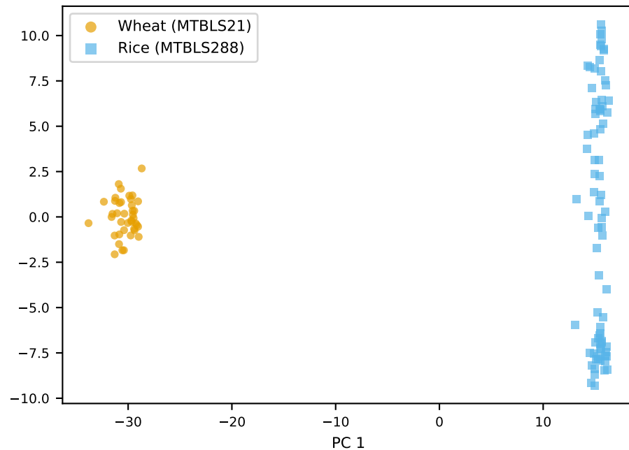
Drift encoder
