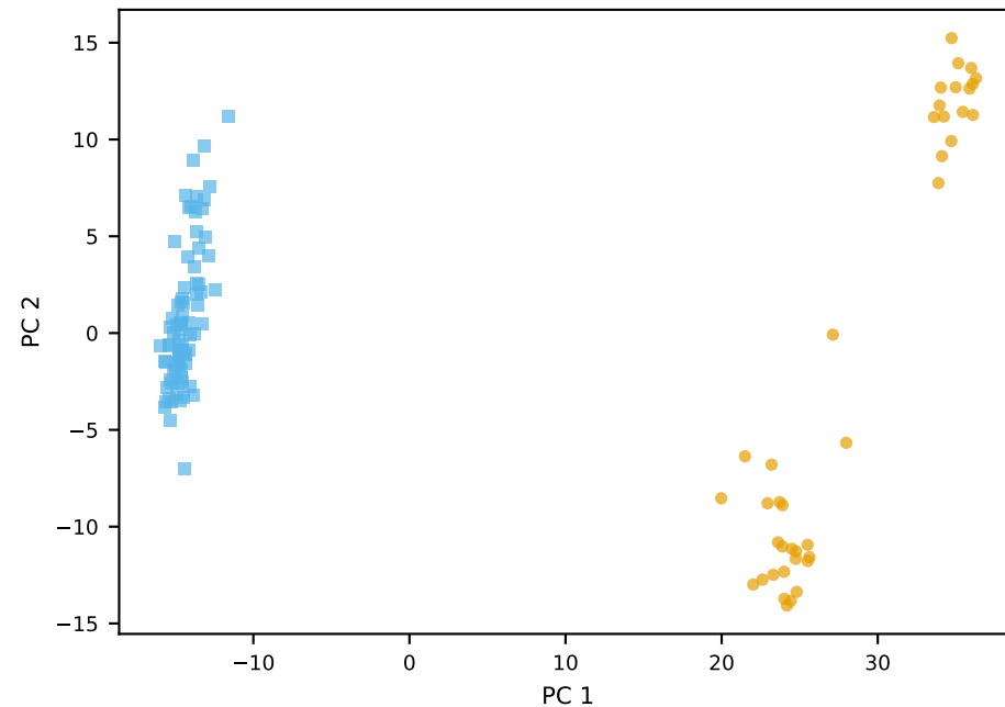
Cross-study encoder
