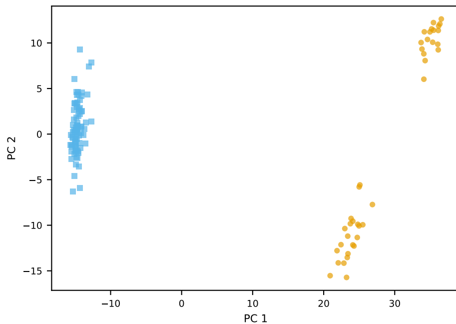
Drift encoder
