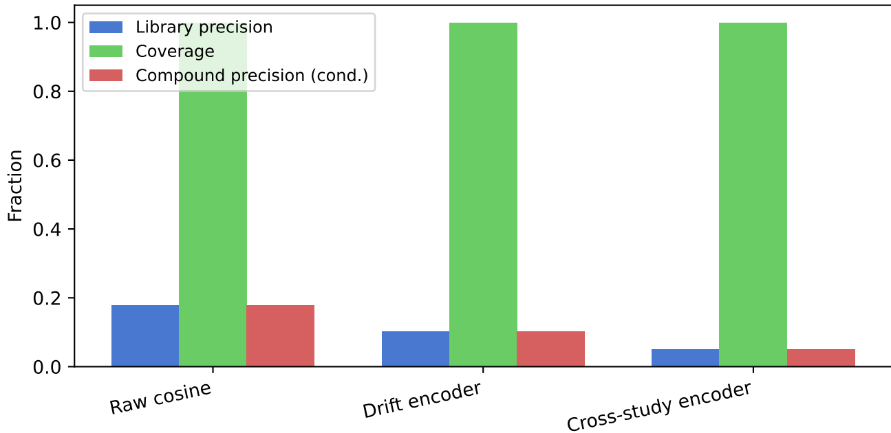
MoNA Library-Matched Compound Precision wheat (MTBLS21) \times rice (MTBLS288), 3,160 pairs
