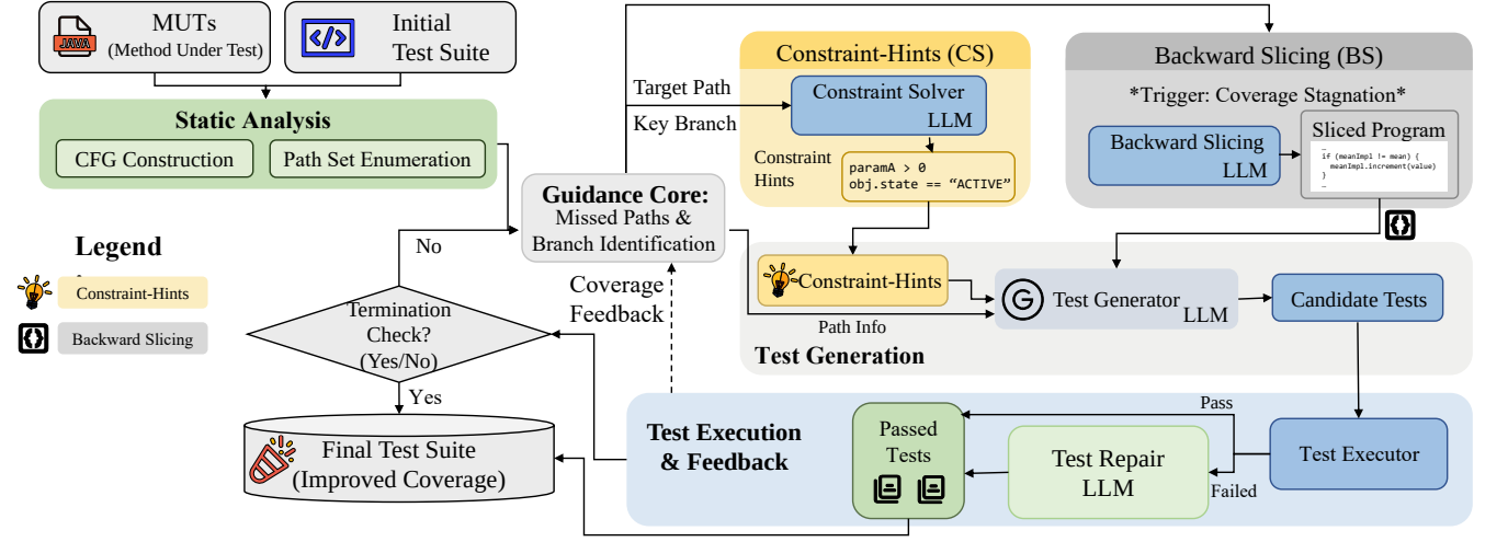
Figure 1: Overview of the coverage-guided test generation framework.
