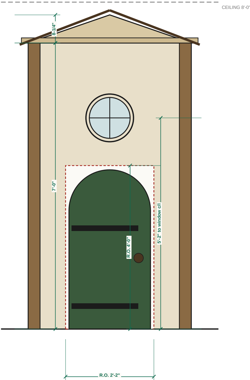
SOUTH ELEVATION (faces the room)
