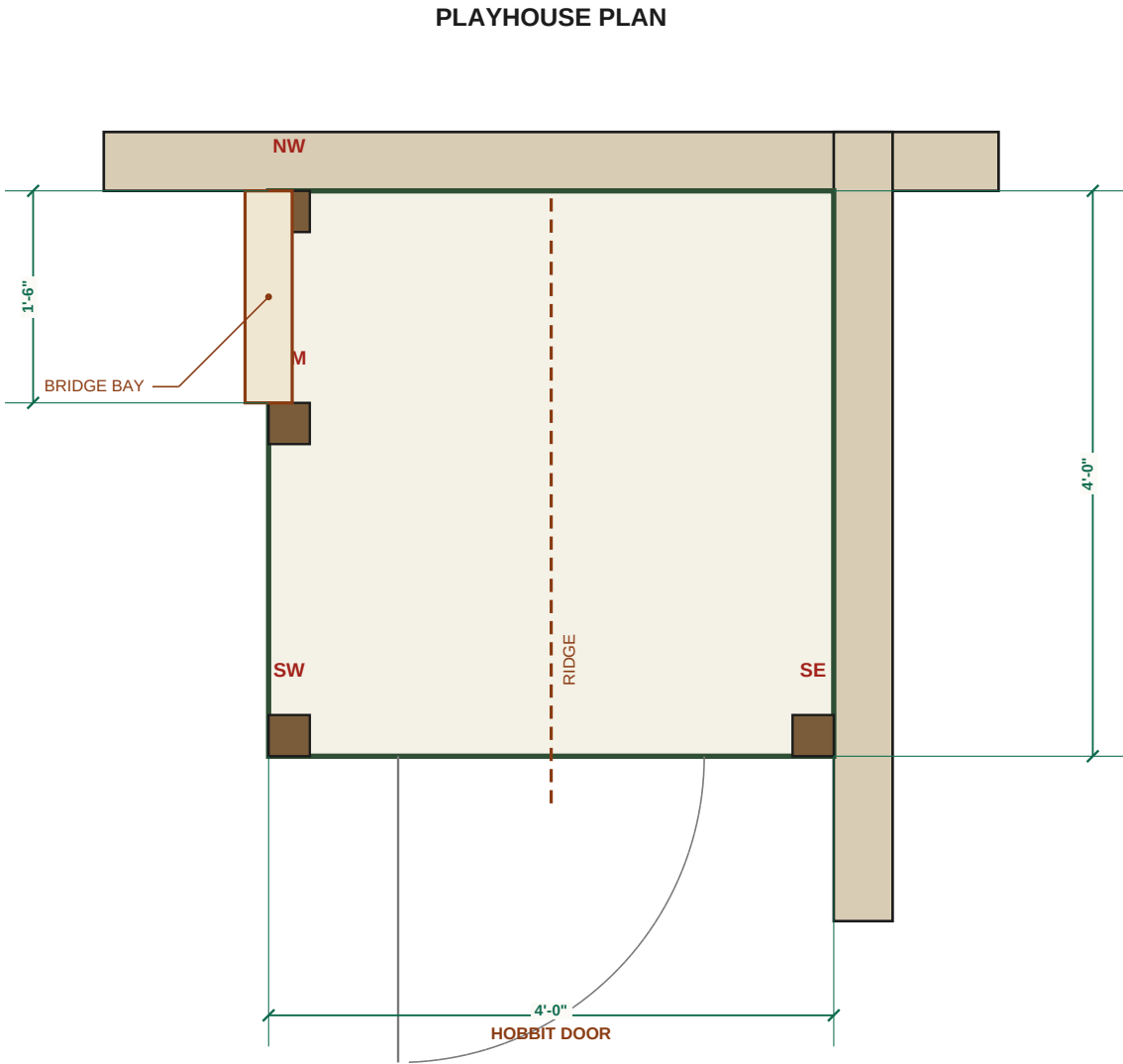
PLAYHOUSE PLAN
