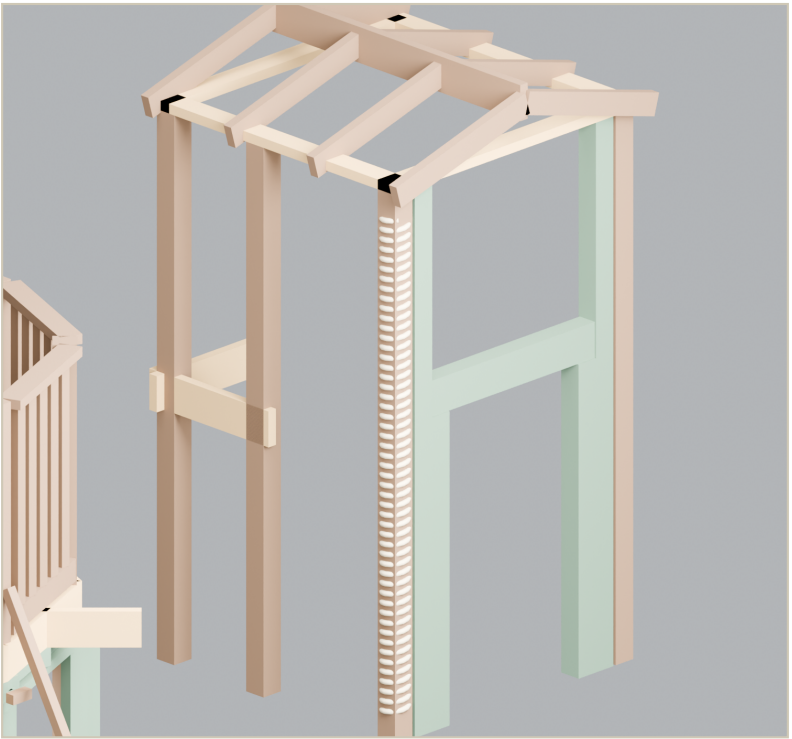
T4 Playhouse framing only — posts, plates, rafters, door bucks
