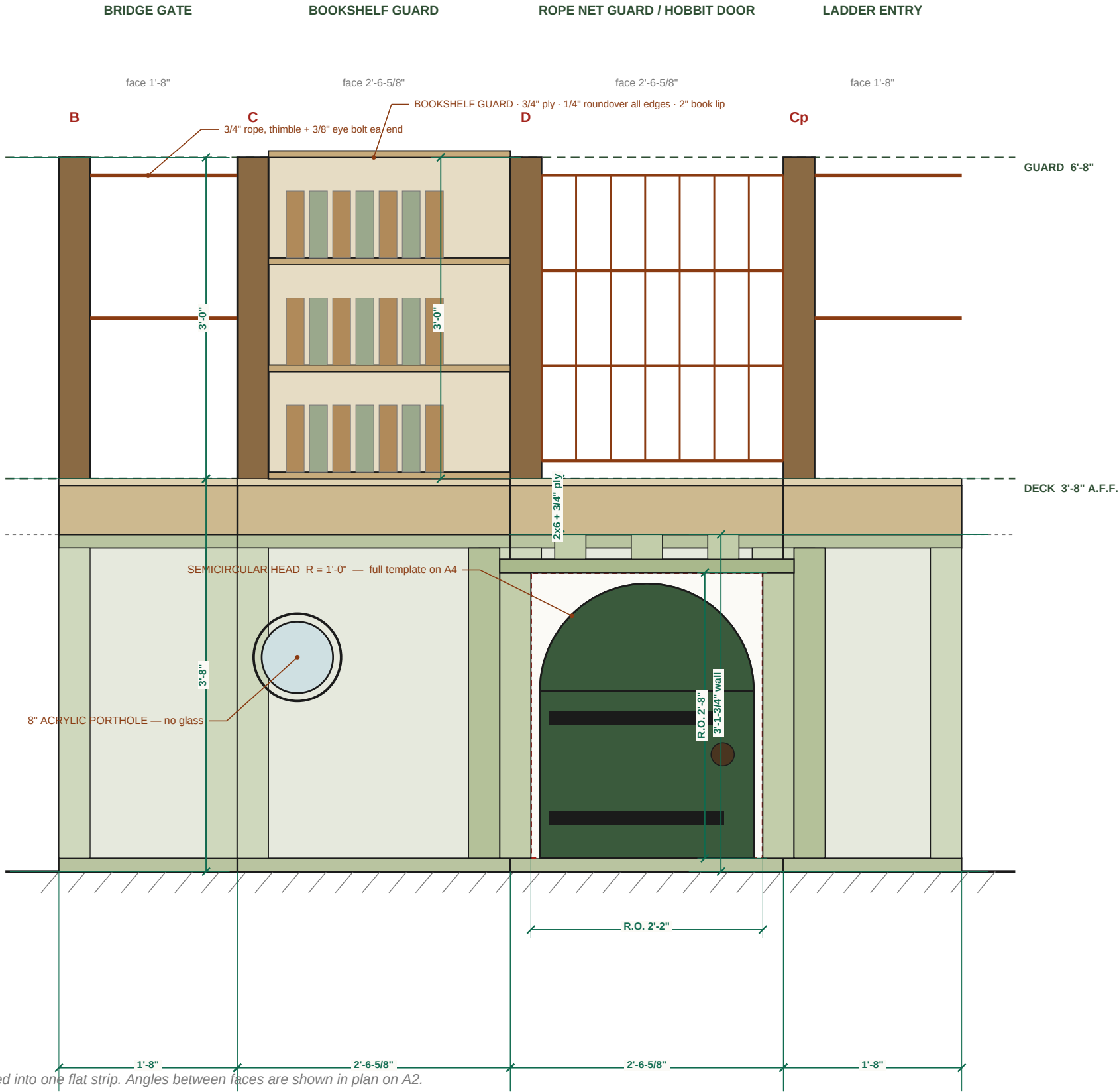
DEVELOPED ELEVATION — the four open faces of the loft unrolled into one flat strip. Angles between faces are shown in plan on A2.
