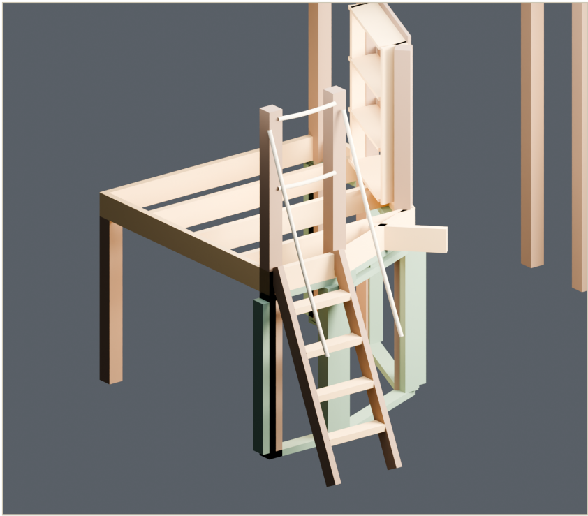
T3 Loft framing only — skins, decking and all rope hidden
