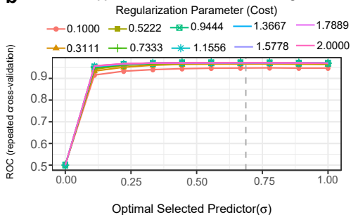
b Support Vector Machine model Training
