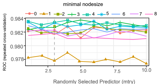
d RandomForest model Training
