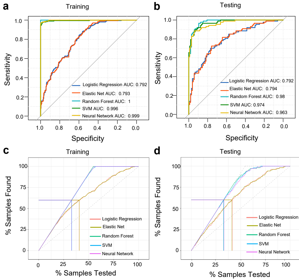
Figure 7. ROC and lift curves of classification models: (a, b) SVM, random forest and neural network models have high AUC value approximate to one in both datasets, while logistic regression and elastic net regularized regression model have similar performance which are worse than the above models. (c, d) Lift defined as how much of an identified population is captured at a given percentile, for a given percentile cutoff what is the proportion of positives were identified over how many positives were identified by the model. Lift curves follows the same pattern as the ROC curves.
