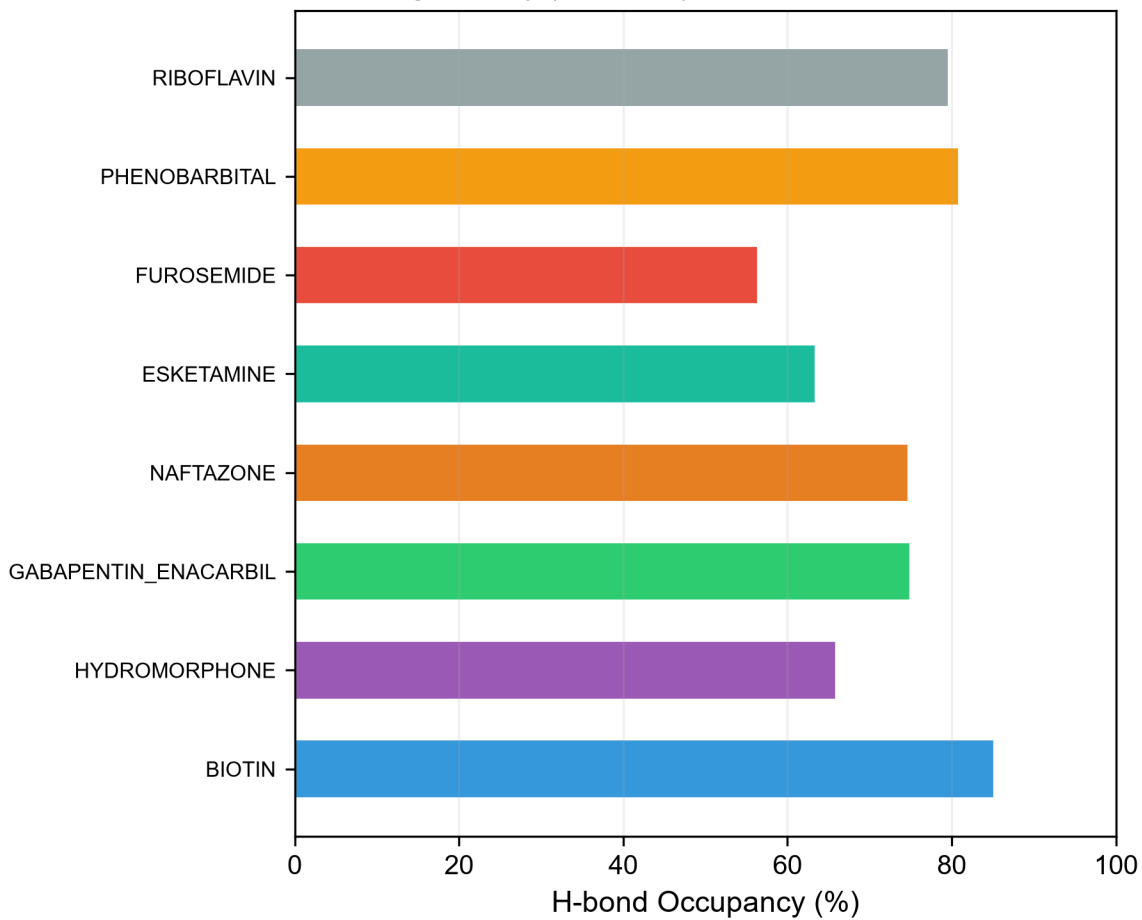
e. Binding Stability (H-bond%)
