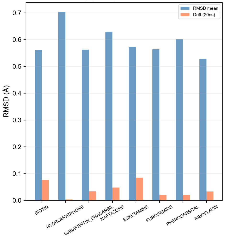
f. Structural Stability (RMSD)
