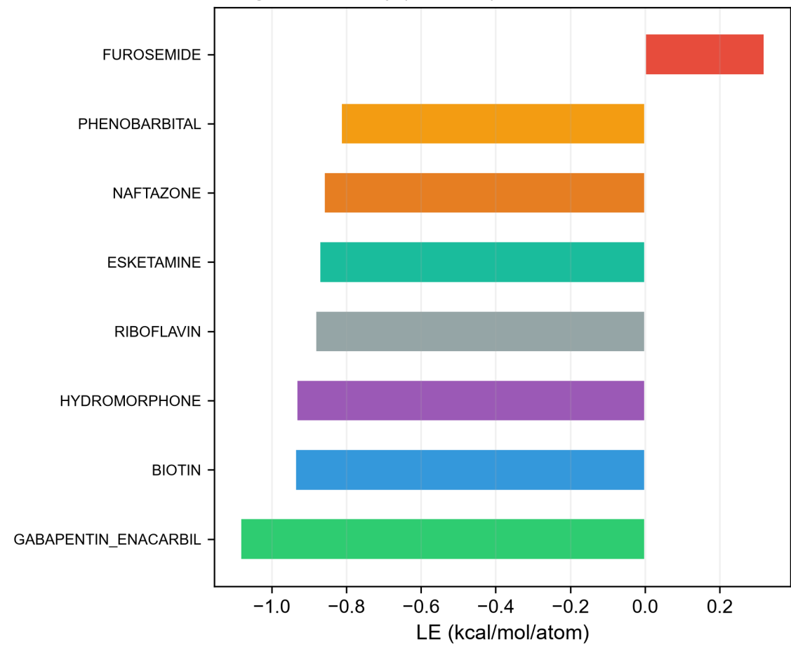
d. Ligand Efficiency (ΔG/atom)
