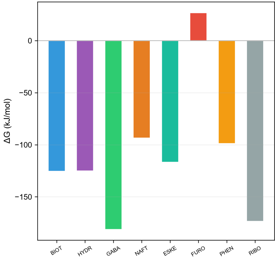
b. MM-GBSA by Compound
