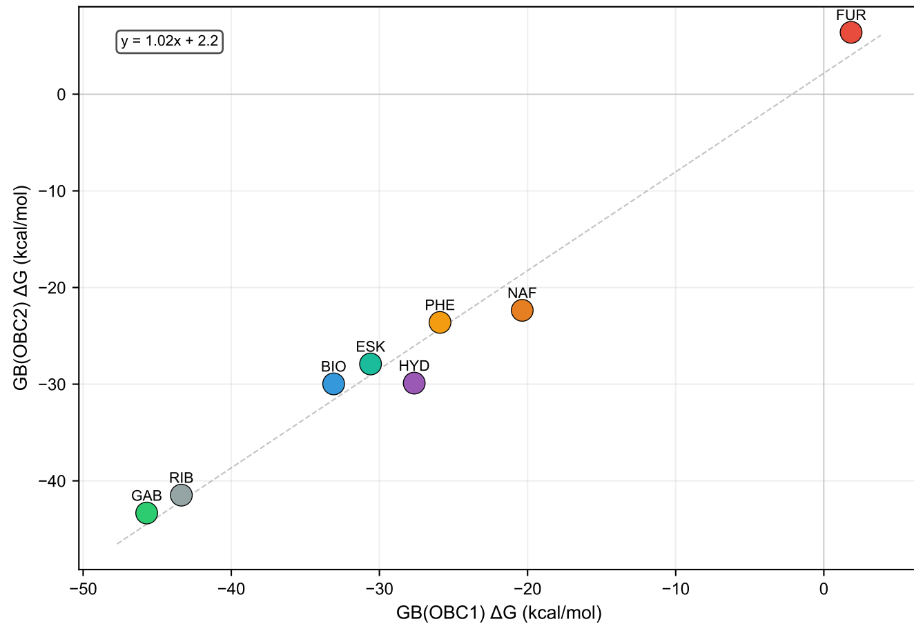
a. Correlation ( R^2=0.975 , Spearman \rho=0.976 )
