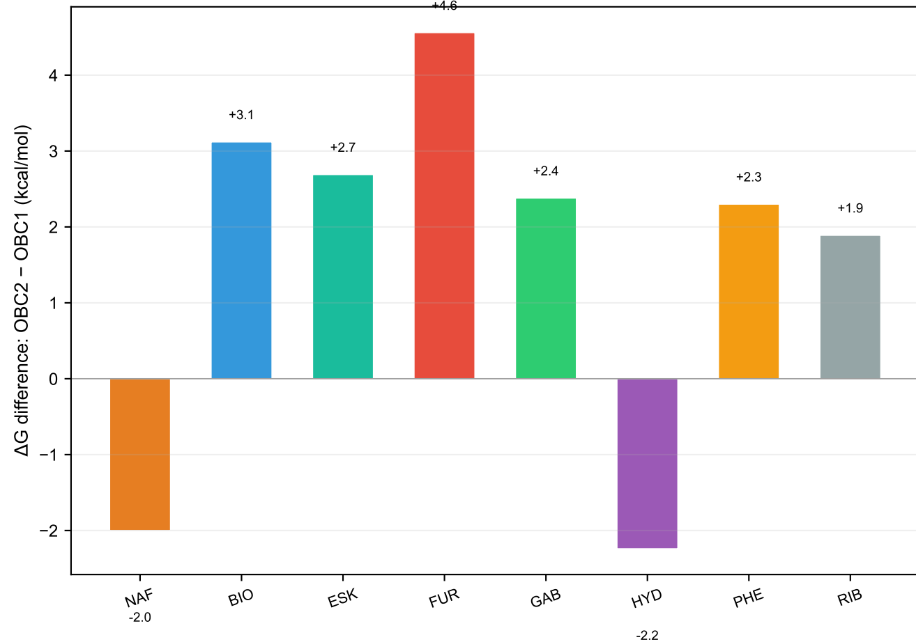
b. Model deviation (RMSD=2.3 kcal/mol)
