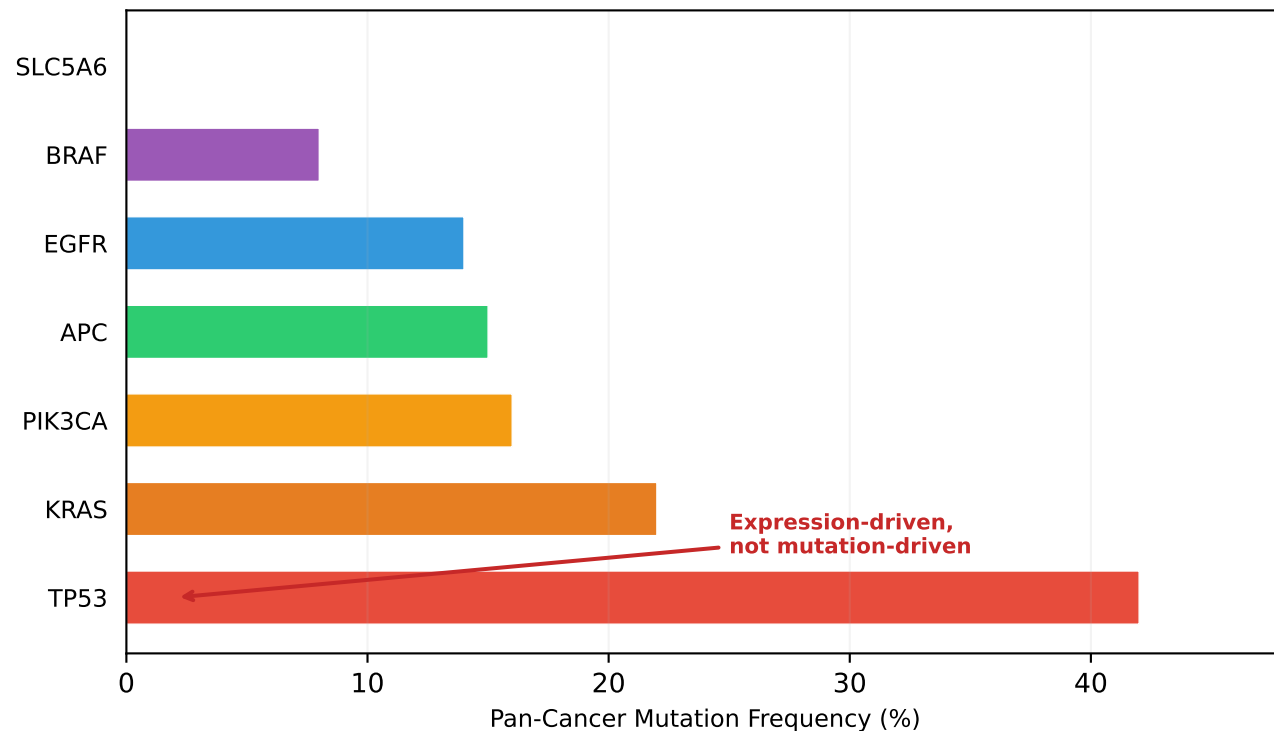
c SLC5A6 vs Known Cancer Genes
