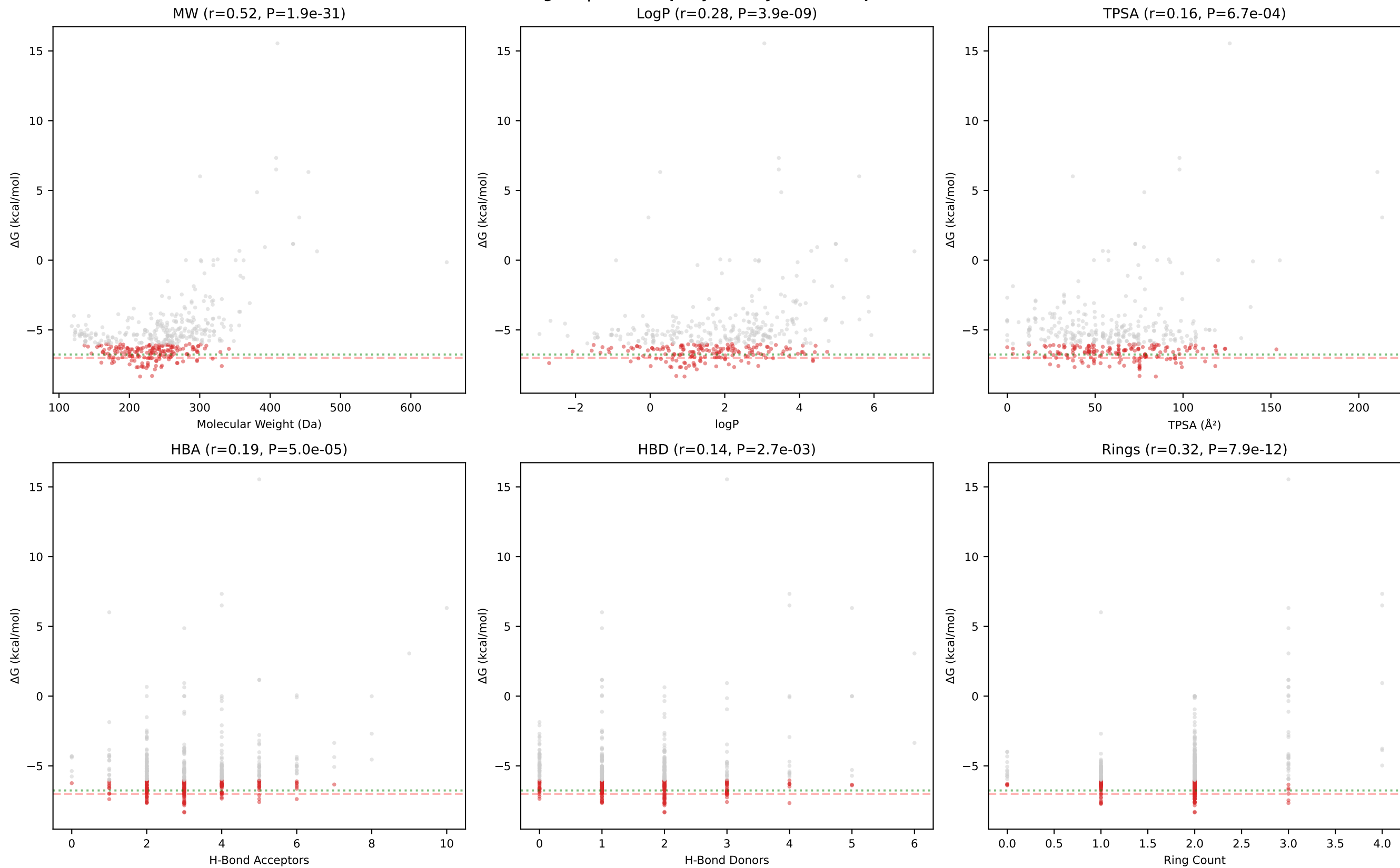
Fig. S6 | SMVT Property-Activity Relationships
