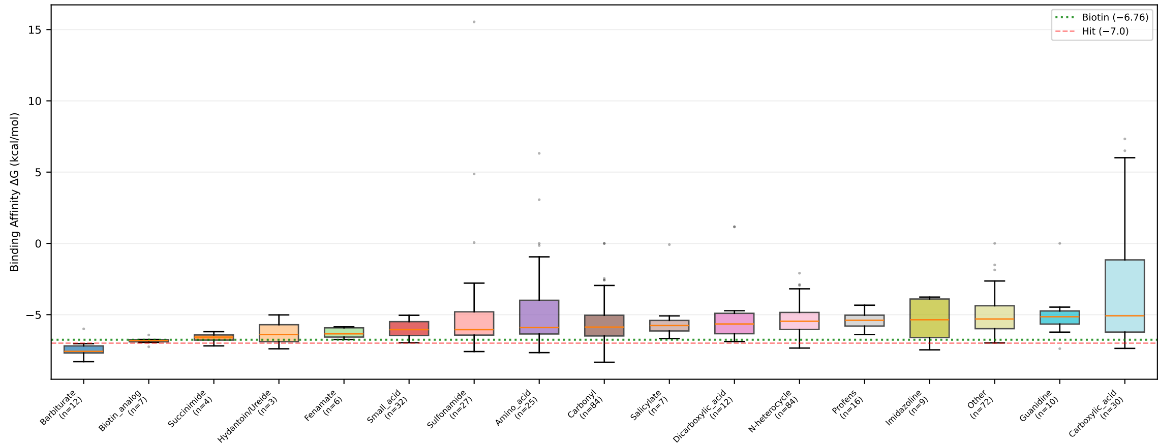
Fig. S7 | Substructure Family SAR Summary
