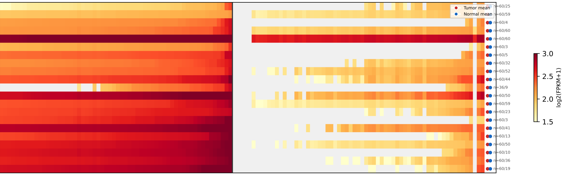
c SLC5A6 Expression
