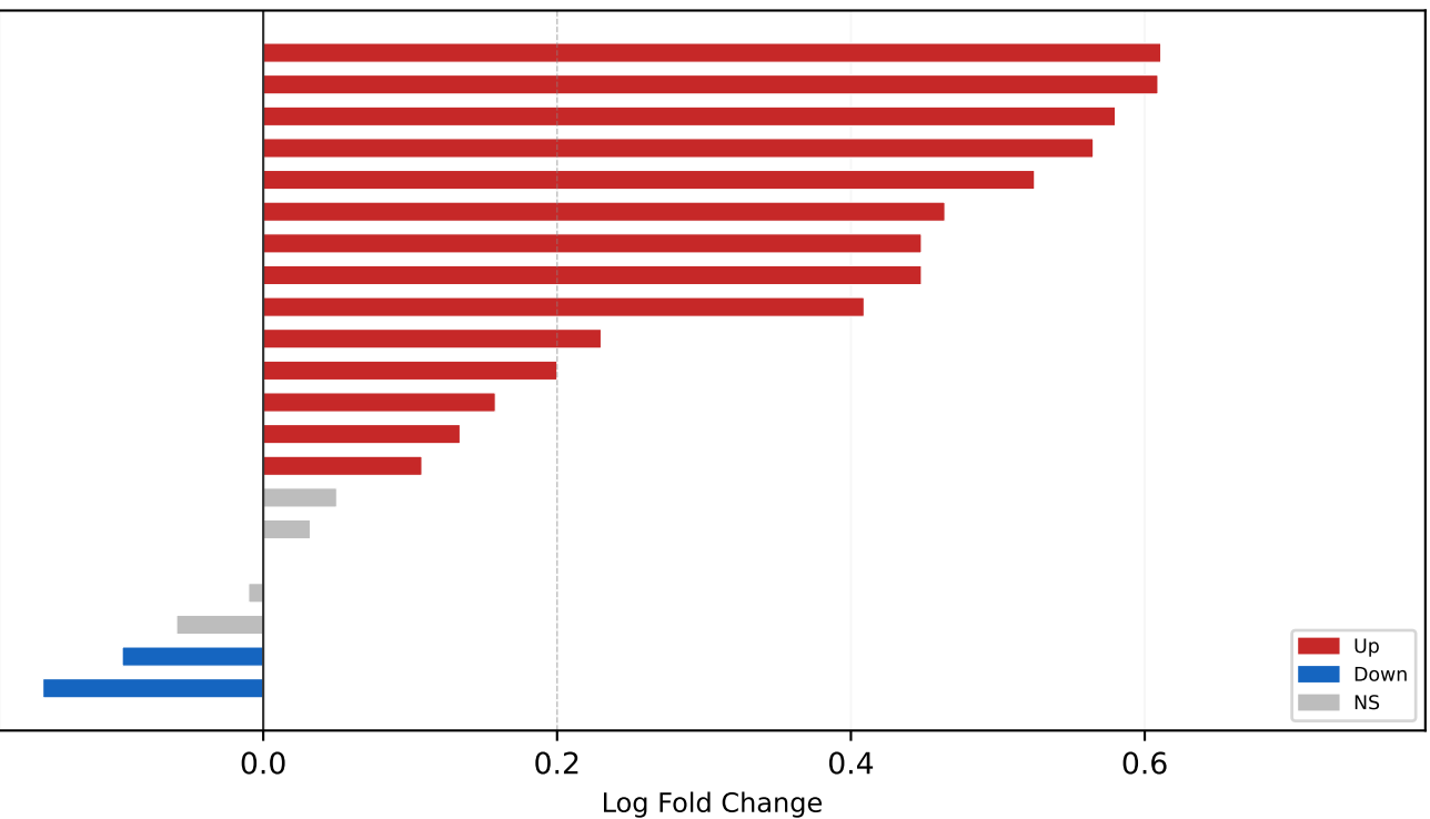
a SLC5A6 Differential Expression
