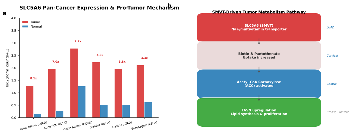
Figure 8: Proposed SLC5A6 pro-tumorigenic mechanism. SMVT-mediated biotin uptake \rightarrow ACC activation \rightarrow de novo fatty acid synthesis \rightarrow tumor proliferation, with HLCS-H4K12bio feedback and PDZD11 membrane anchoring.
