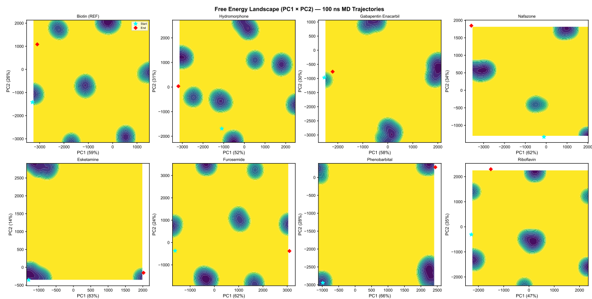
Figure 18: Free energy landscape (PC1 × PC2).
