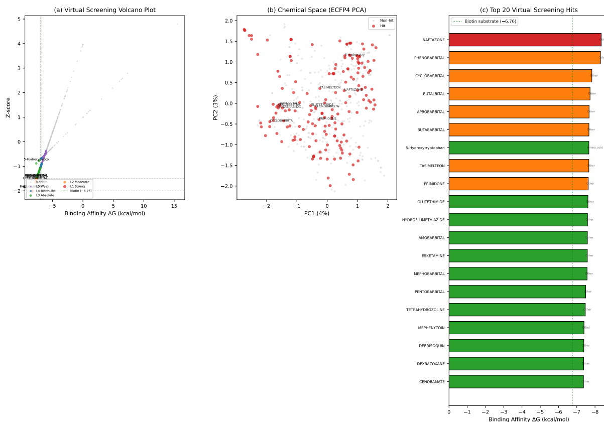
Figure 6: Virtual screening results. (a) Volcano plot of all 440 docked compounds. (b) Chemical space PCA. (c) Top 20 hits with clinical annotation.
