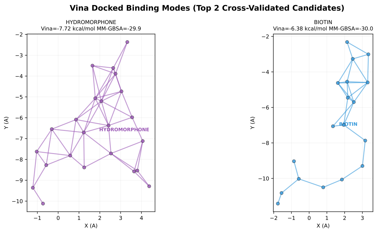
Figure 17: Binding mode visualisation.
