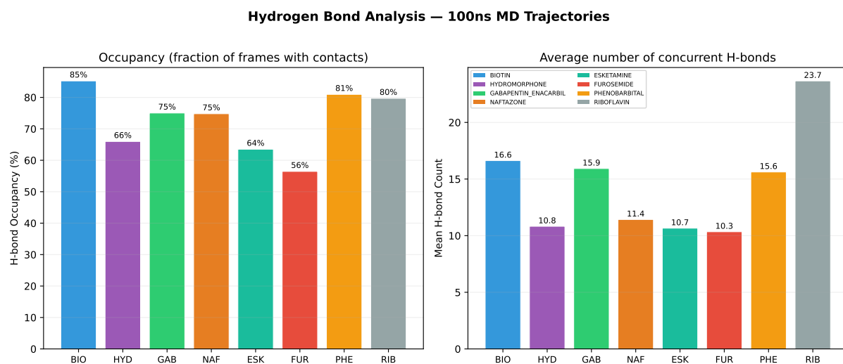
Figure 15: Hydrogen bond analysis.
