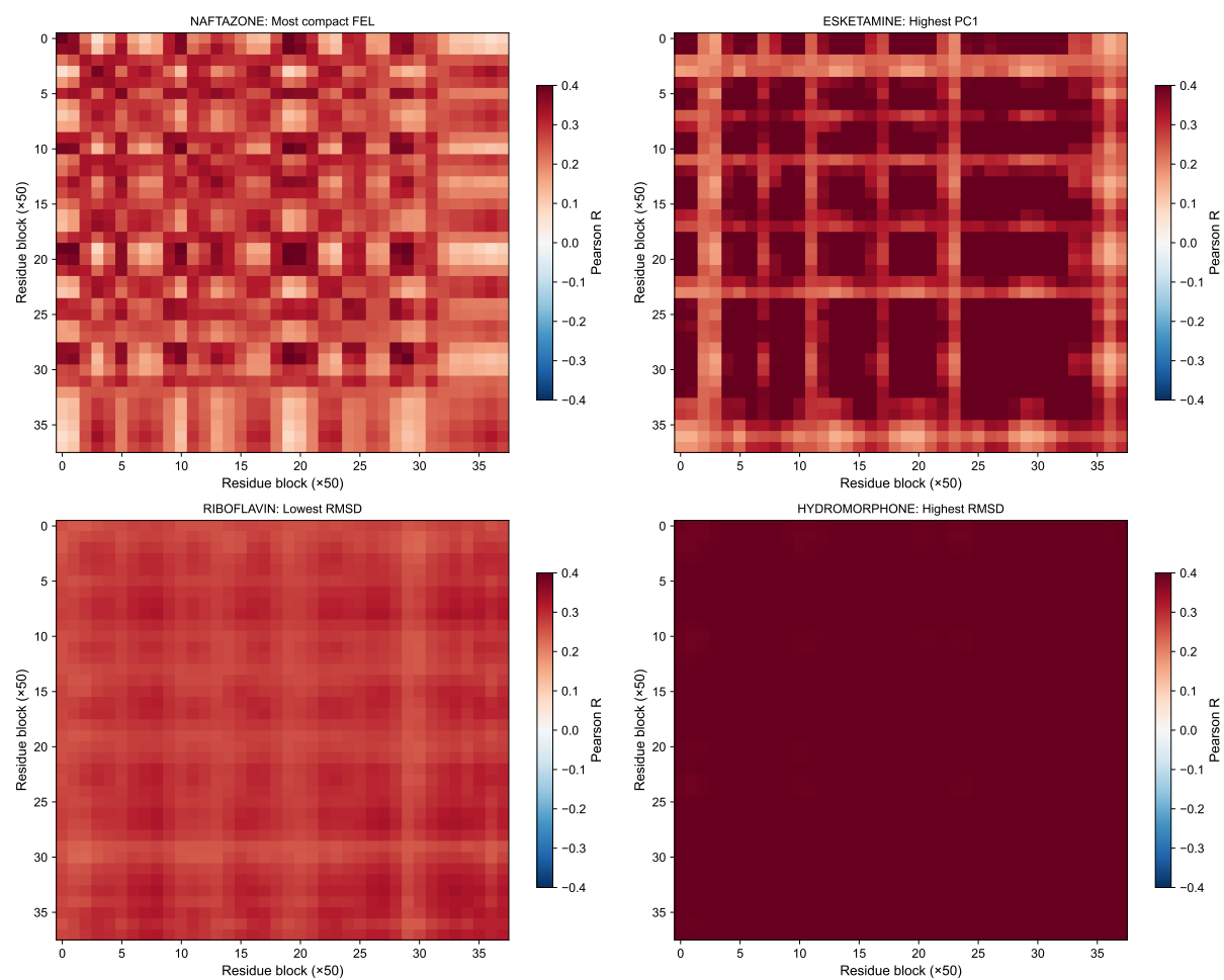
Figure 19: Dynamic cross-correlation matrices.
