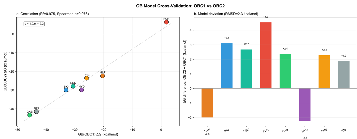
Figure 22: GB model cross-validation (OBC1 vs OBC2).
