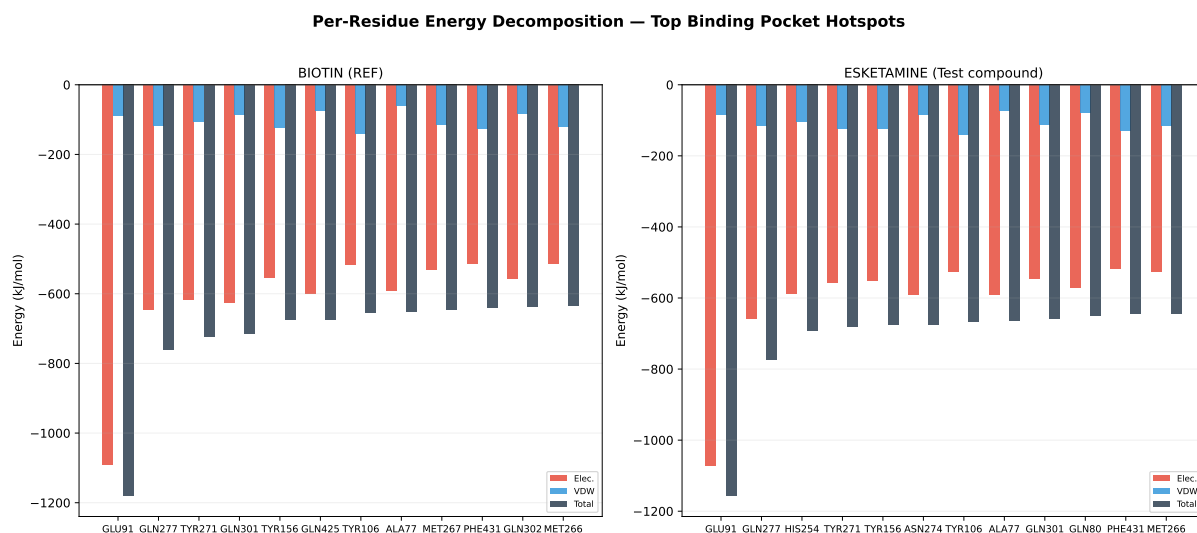
Figure 14: Per-residue energy decomposition.
