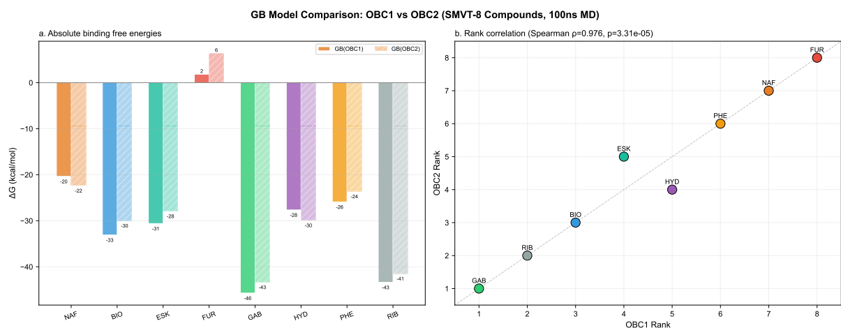
Figure 21: GB model comparison (OBC1 vs OBC2).
