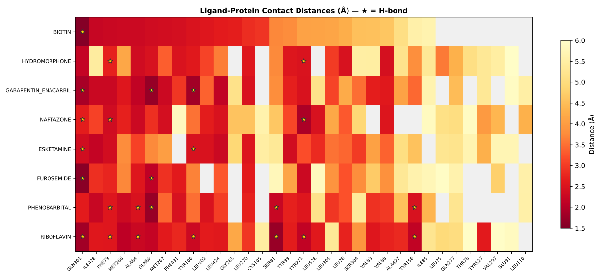
Figure 16: Ligand-protein contact distance heatmap.
