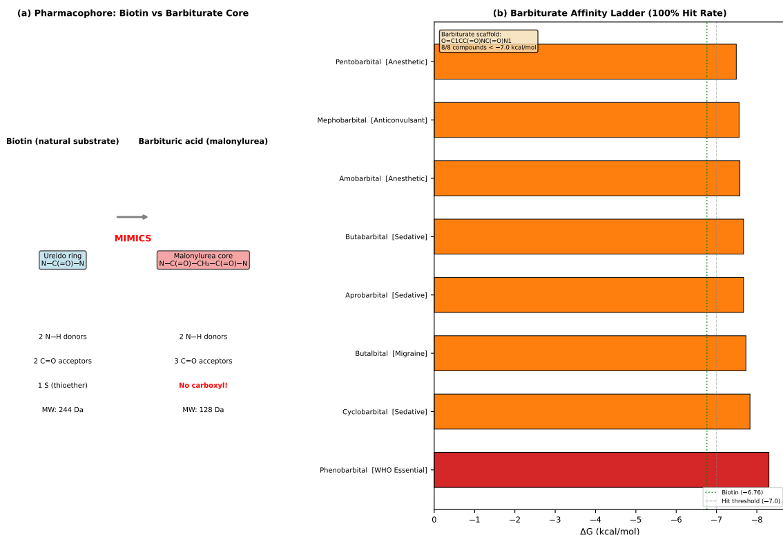
Figure 7: Barbiturate pharmacophore. (a) Structural comparison of biotin ureido ring vs. barbituric acid malonylurea core. (b) Affinity ladder showing 100% barbiturate hit rate.
