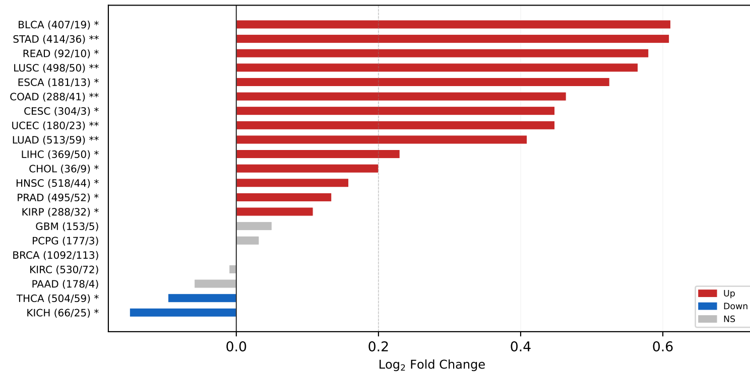
a Differential Expression
