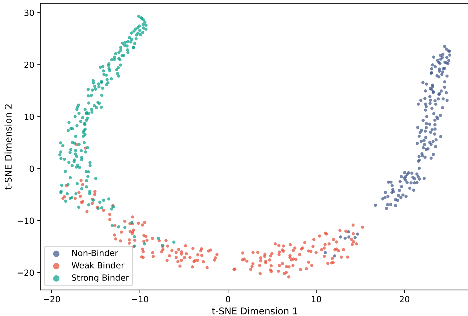
t-SNE of Penultimate-Layer Features Colored by True Class (SB / WB / NB)
