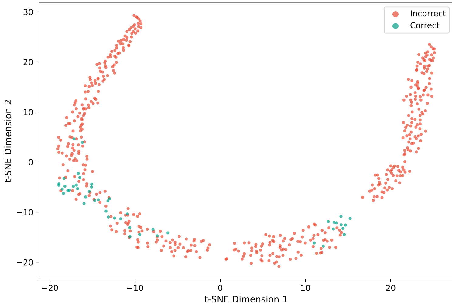
t-SNE of Penultimate-Layer Features Colored by Prediction Correctness
