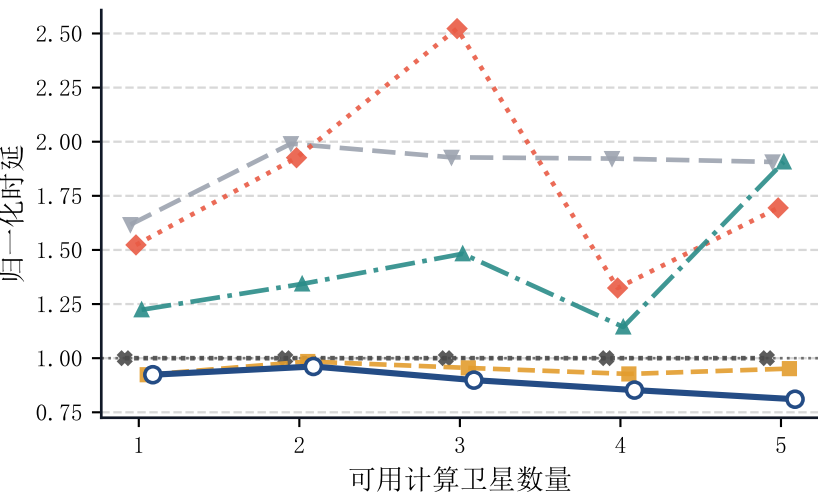
Swin-Base
