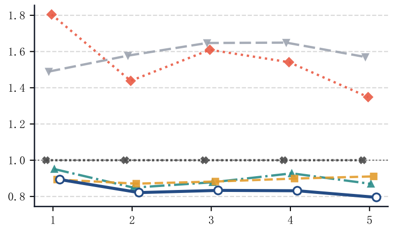
ResNet101
