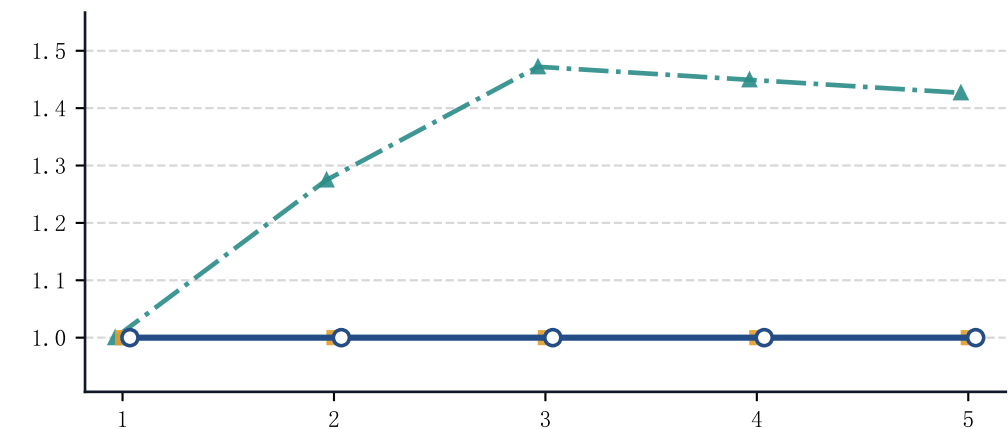
Swin-Base
