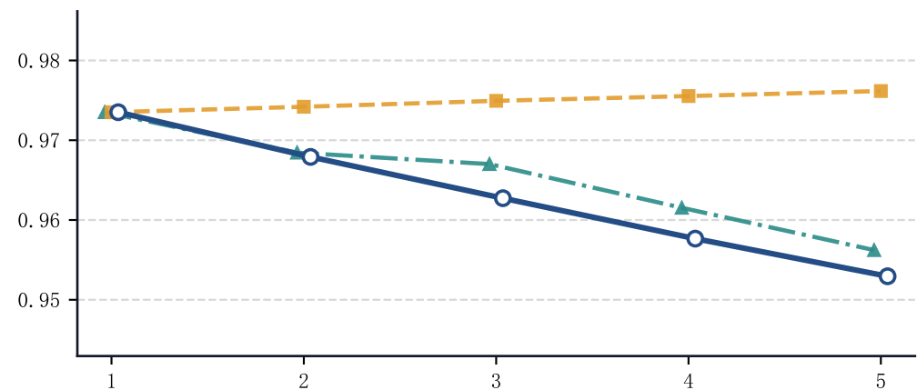
ResNet101
