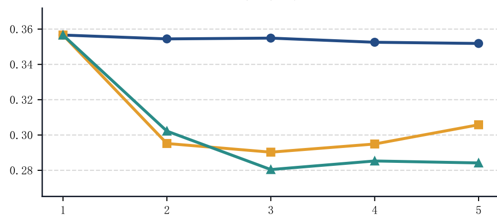
ResNet101
