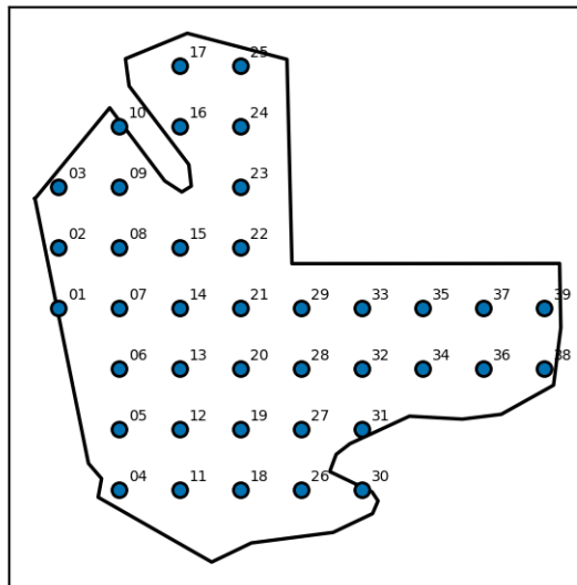
Unit 115 plots, 300 ft grid (orange: QA flag)
