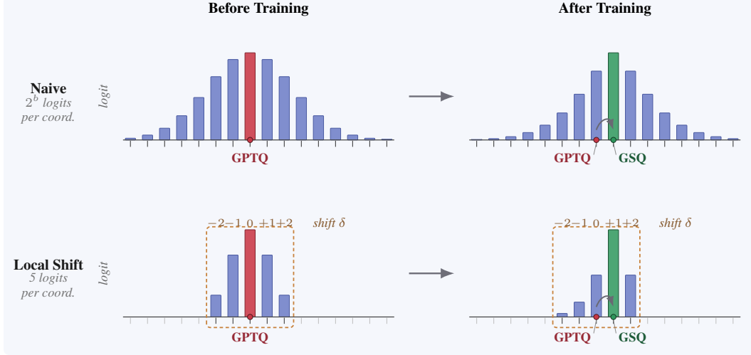
Figure 1: Local-shift parameterization at higher bit-widths. Each row shows, for a single weight coordinate, the logit distribution over candidate grid points before and after training. The red bar and dot mark the GPTQ-initialized grid point used to warm-start the logits; the green bar and dot mark the grid point selected by GSQ after training. Top (naive) : placing one trainable logit on every grid point costs 2^b logits per coordinate, which quickly becomes prohibitive as b grows. Bottom (local shift) : we instead assign logits only to a discrete shift \delta_i \in \{-2, -1, 0, +1, +2\} relative to the GPTQ-initialized grid index (dashed window), reducing the per-coordinate parameter count from 2^b to 5. In both cases the distribution is initialized as a Gaussian centered at the GPTQ solution.
