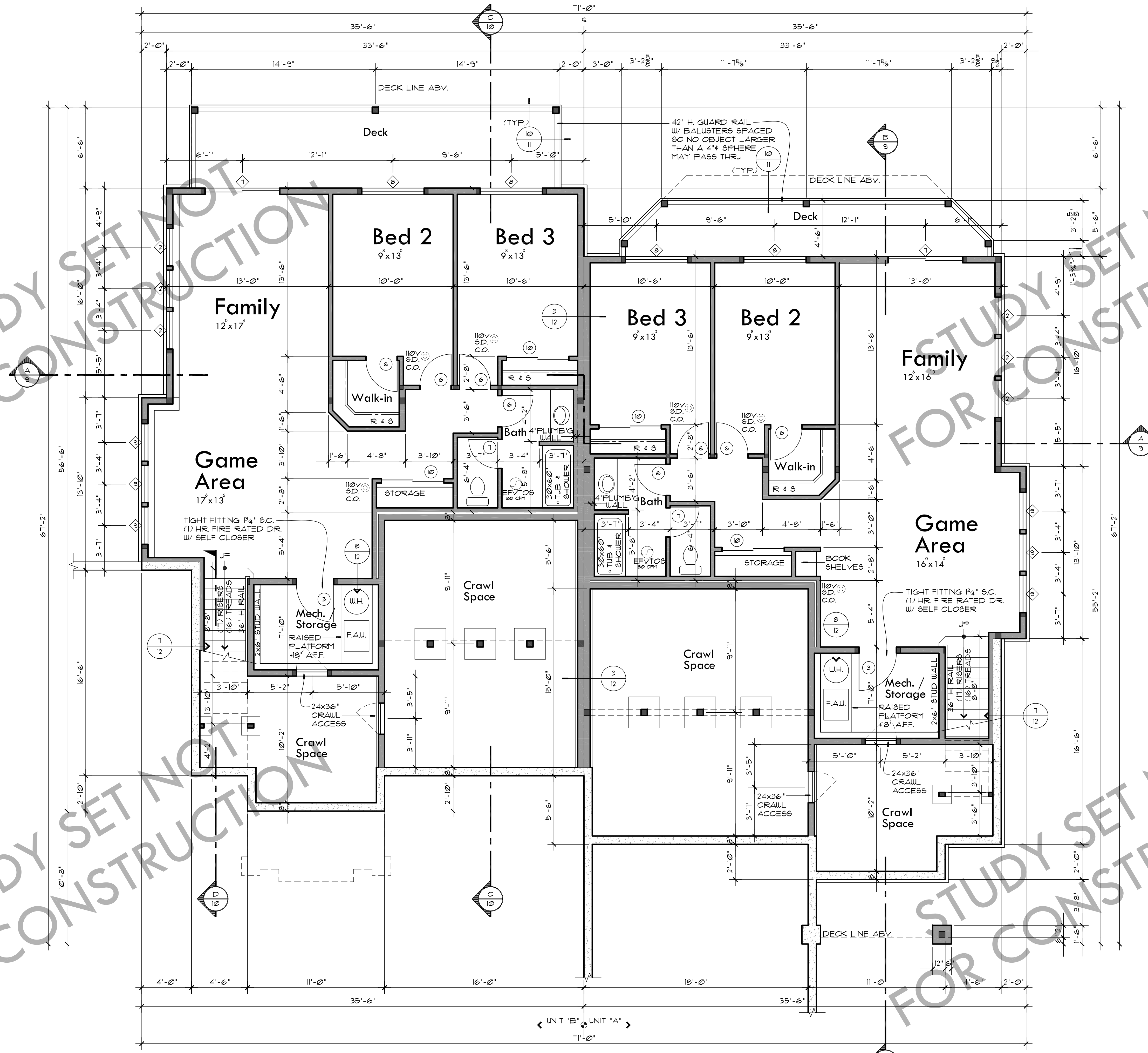
LOWER FLOOR PLAN
