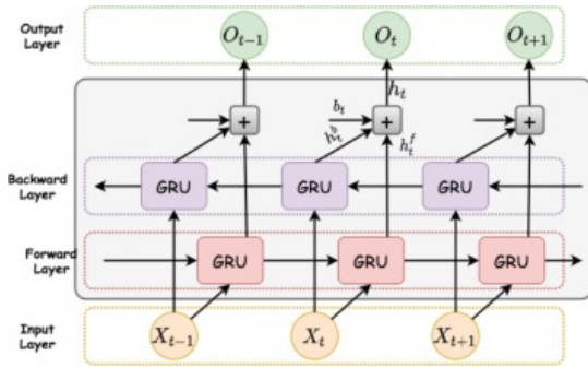
Fig. 6. Bidirectional GRU structure showing forward and backward processing
