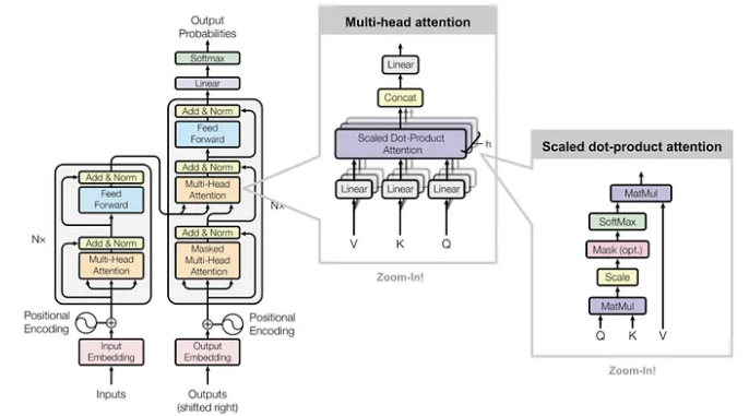
Fig. 8. Transformer Architecture
