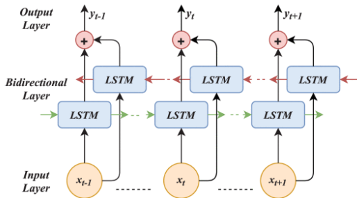
Fig. 3. Structure of BiLSTM showing forward and backward LSTM layers combines forward and backward LSTM layers, each process-
