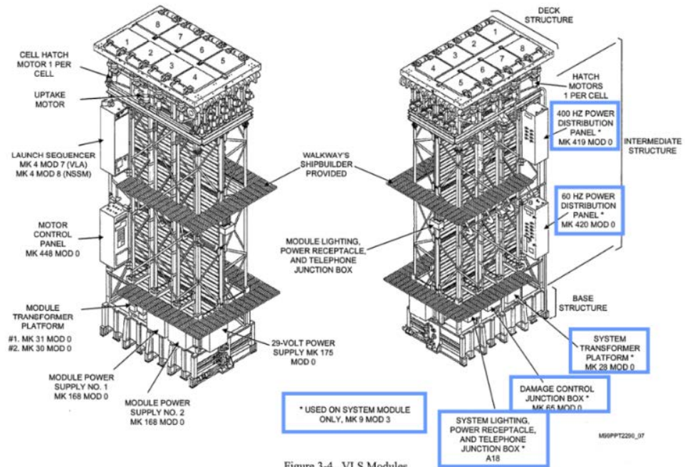
Figure 3-4. VLS Modules
