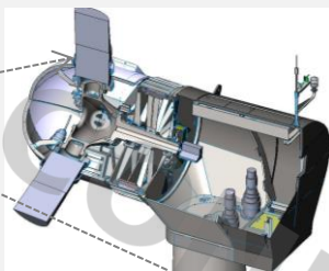
[DMS200_200kW 풍력기]
