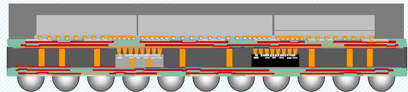
Key Tech Si(w/TSV)&Molded bridge, Double side RDL
