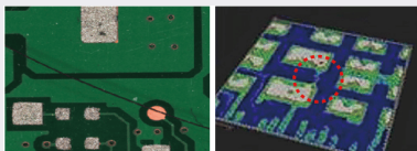
3D SPI (Solder Paste Inspection)
