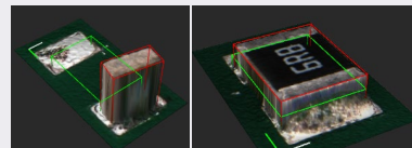
3D AOI (Automated Optical Inspection)
