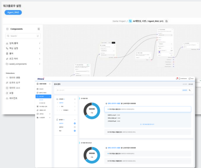
Athena Platform
