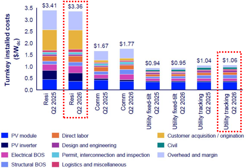
US national average system prices by market segment
