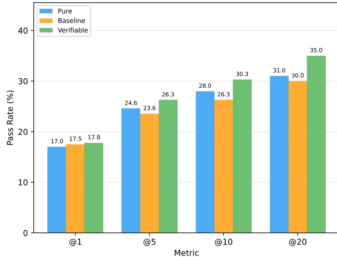
Figure 1: Pass@K Performance Comparison Across Benchmarks
