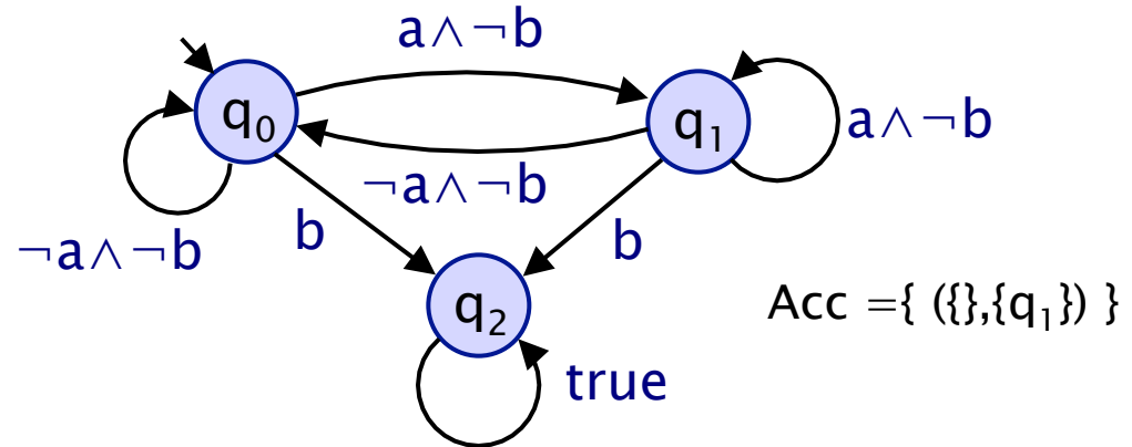
DRA A_\psi for \psi = \mathbf{G}\neg b \wedge \mathbf{GF} a
